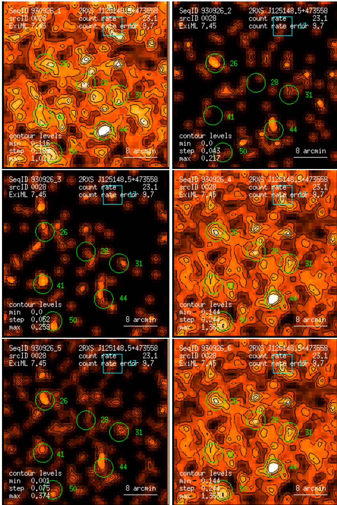
Figure 28: RASS 930926: detection 0028: band rate images, Gaussian filter: (1) PSPC channels 11 – 41, (2) 52 – 90, (3) 91 – 201, (4) 11 – 235, (5) 52 – 201, (6) 11 – 201. Broad band rates in counts/ks. Band rate contour levels in counts/ks/arcmin 2 .
