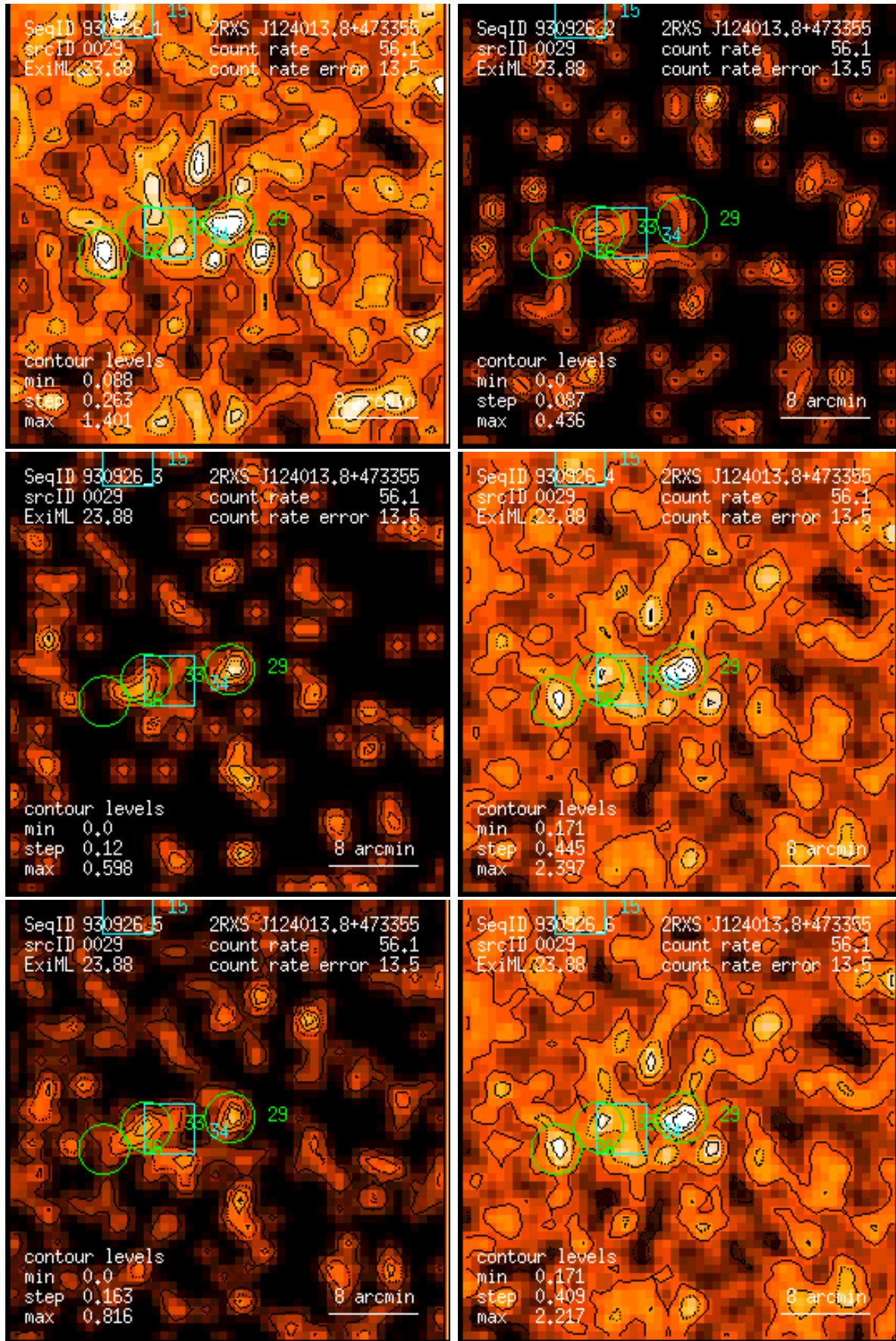
Figure 29: RASS 930926: detection 0029: band rate images, Gaussian filter: (1) PSPC channels 11 – 41, (2) 52 – 90, (3) 91 – 201, (4) 11 – 235, (5) 52 – 201, (6) 11 – 201. Broad band rates in counts/ks. Band rate contour levels in counts/ks/arcmin 2 .
