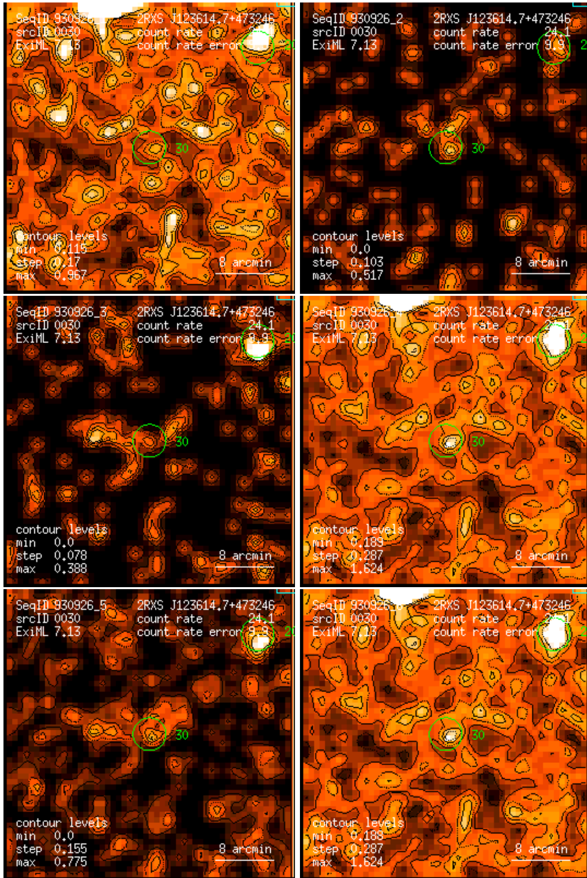
Figure 30: RASS 930926: detection 0030: band rate images, Gaussian filter: (1) PSPC channels 11 – 41, (2) 52 – 90, (3) 91 – 201, (4) 11 – 235, (5) 52 – 201, (6) 11 – 201. Broad band rates in counts/ks. Band rate contour levels in counts/ks/arcmin 2 .
