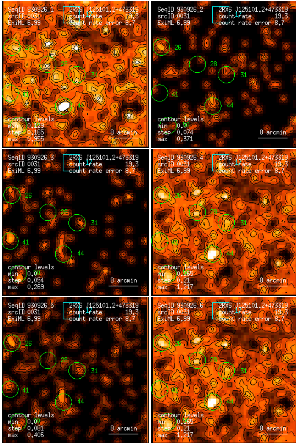
Figure 31: RASS 930926: detection 0031: band rate images, Gaussian filter: (1) PSPC channels 11 – 41, (2) 52 – 90, (3) 91 – 201, (4) 11 – 235, (5) 52 – 201, (6) 11 – 201. Broad band rates in counts/ks. Band rate contour levels in counts/ks/arcmin 2 .
