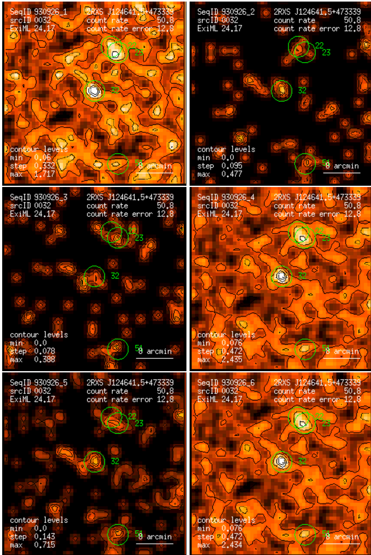
Figure 32: RASS 930926: detection 0032: band rate images, Gaussian filter: (1) PSPC channels 11 – 41, (2) 52 – 90, (3) 91 – 201, (4) 11 – 235, (5) 52 – 201, (6) 11 – 201. Broad band rates in counts/ks. Band rate contour levels in counts/ks/arcmin 2 .
