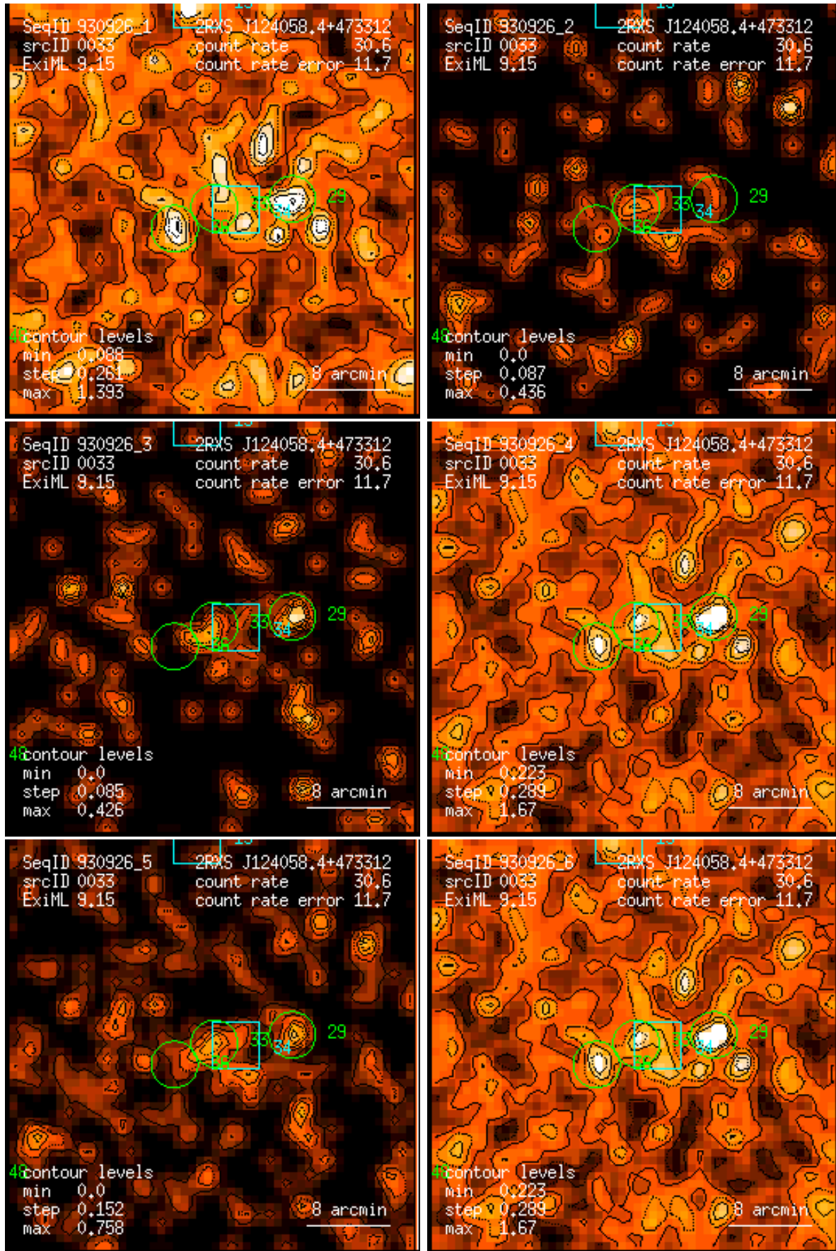
Figure 33: RASS 930926: detection 0033: band rate images, Gaussian filter: (1) PSPC channels 11 – 41, (2) 52 – 90, (3) 91 – 201, (4) 11 – 235, (5) 52 – 201, (6) 11 – 201. Broad band rates in counts/ks. Band rate contour levels in counts/ks/arcmin 2 .
