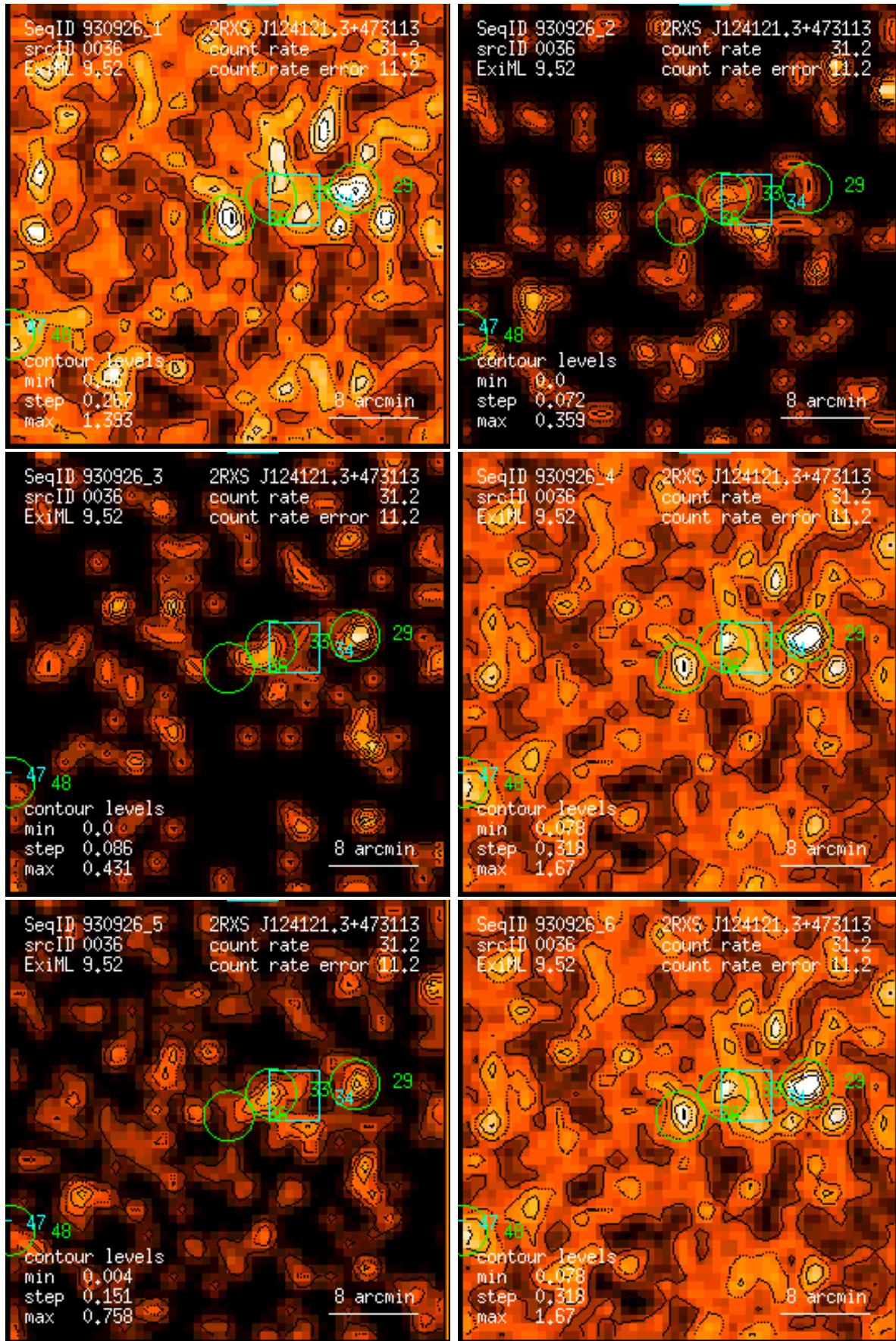
Figure 36: RASS 930926: detection 0036: band rate images, Gaussian filter: (1) PSPC channels 11 – 41, (2) 52 – 90, (3) 91 – 201, (4) 11 – 235, (5) 52 – 201, (6) 11 – 201. Broad band rates in counts/ks. Band rate contour levels in counts/ks/arcmin 2 .
