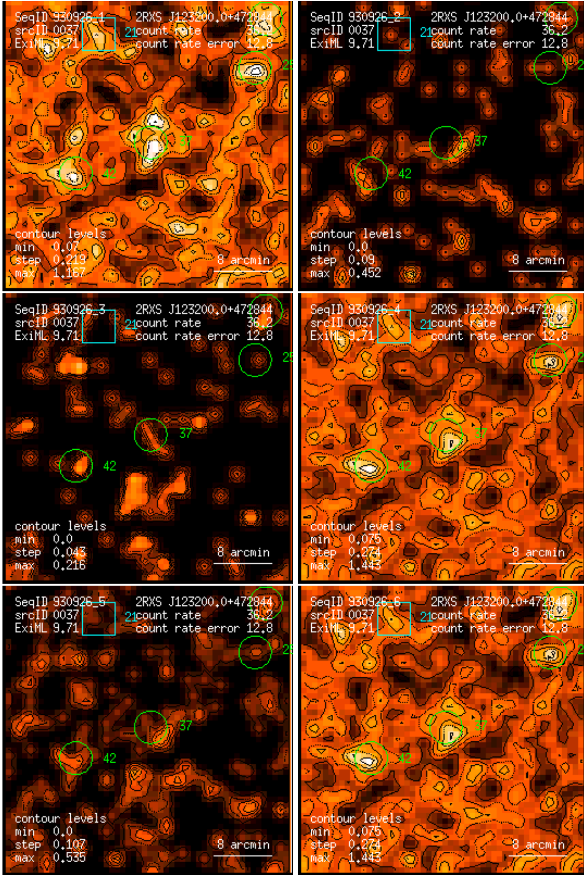
Figure 37: RASS 930926: detection 0037: band rate images, Gaussian filter: (1) PSPC channels 11 – 41, (2) 52 – 90, (3) 91 – 201, (4) 11 – 235, (5) 52 – 201, (6) 11 – 201. Broad band rates in counts/ks. Band rate contour levels in counts/ks/arcmin 2 .
