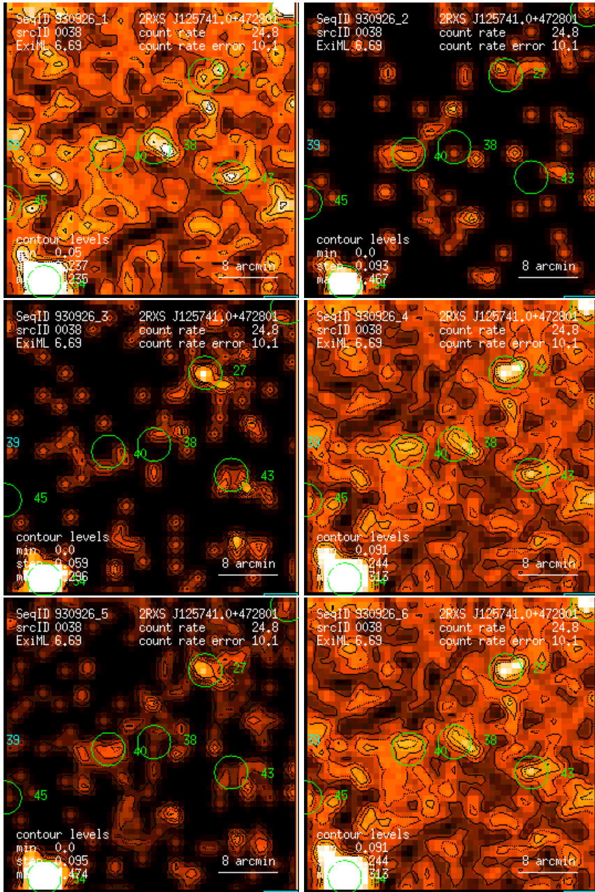
Figure 38: RASS 930926: detection 0038: band rate images, Gaussian filter: (1) PSPC channels 11 – 41, (2) 52 – 90, (3) 91 – 201, (4) 11 – 235, (5) 52 – 201, (6) 11 – 201. Broad band rates in counts/ks. Band rate contour levels in counts/ks/arcmin 2 .
