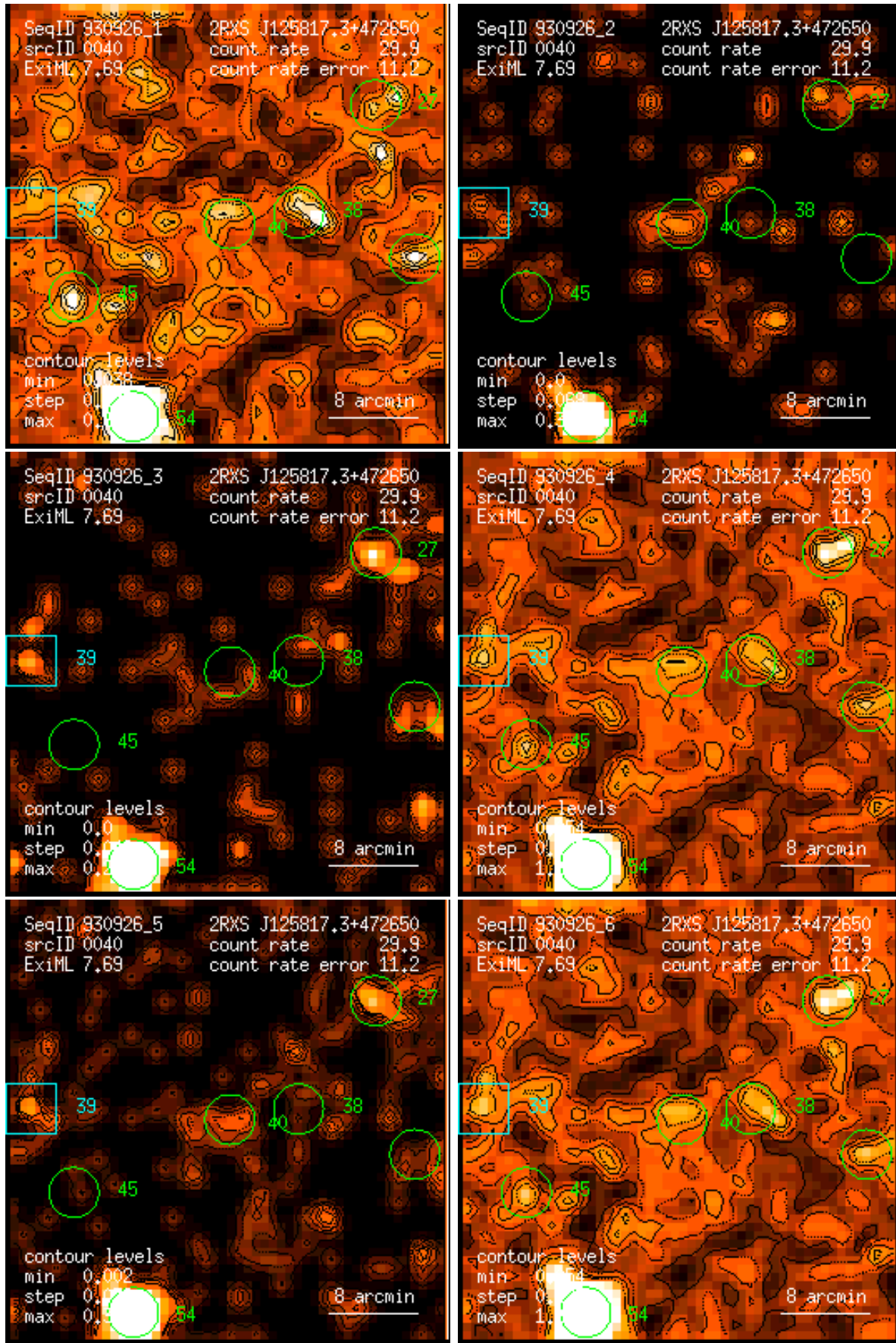
Figure 40: RASS 930926: detection 0040: band rate images, Gaussian filter: (1) PSPC channels 11 – 41, (2) 52 – 90, (3) 91 – 201, (4) 11 – 235, (5) 52 – 201, (6) 11 – 201. Broad band rates in counts/ks. Band rate contour levels in counts/ks/arcmin 2 .
