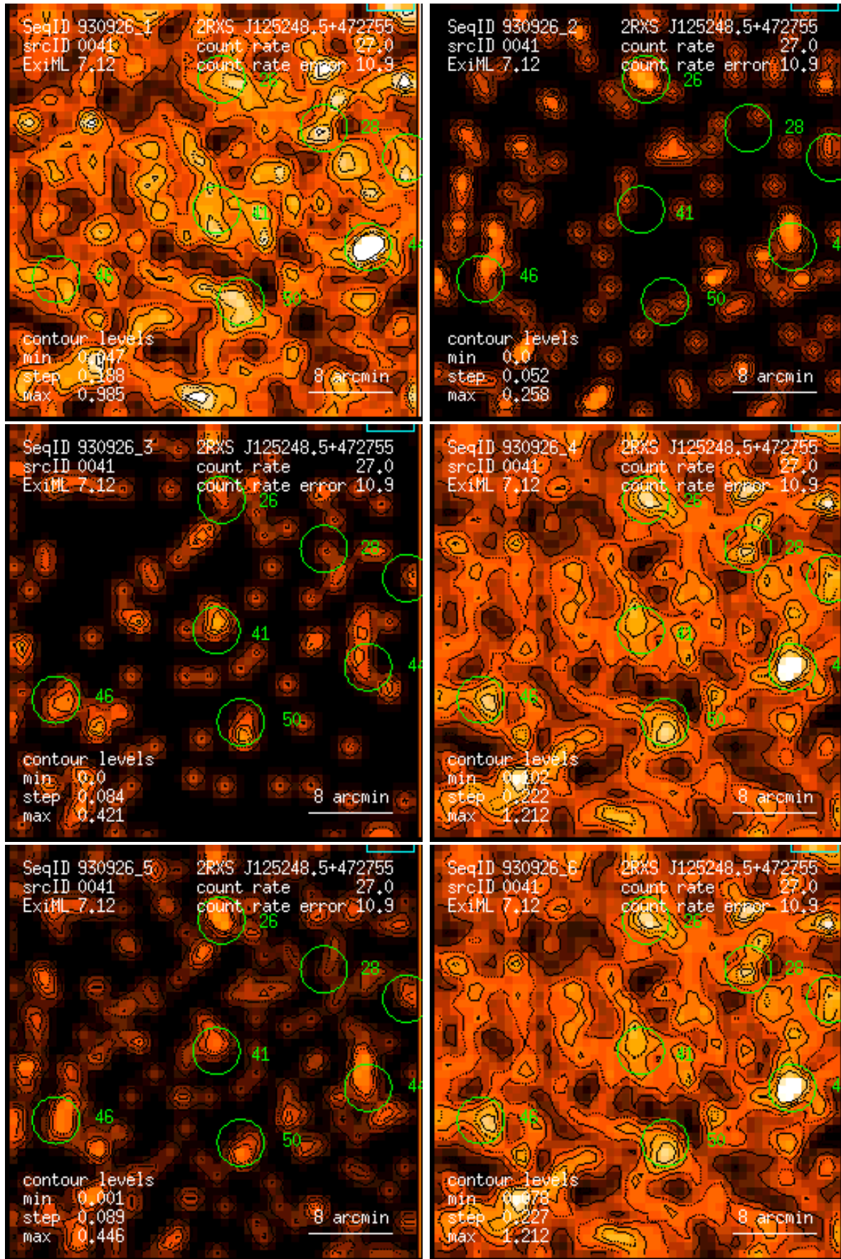
Figure 41: RASS 930926: detection 0041: band rate images, Gaussian filter: (1) PSPC channels 11 – 41, (2) 52 – 90, (3) 91 – 201, (4) 11 – 235, (5) 52 – 201, (6) 11 – 201. Broad band rates in counts/ks. Band rate contour levels in counts/ks/arcmin 2 .
