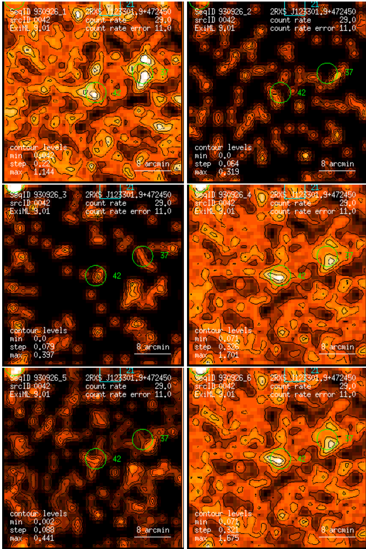
Figure 42: RASS 930926: detection 0042: band rate images, Gaussian filter: (1) PSPC channels 11 – 41, (2) 52 – 90, (3) 91 – 201, (4) 11 – 235, (5) 52 – 201, (6) 11 – 201. Broad band rates in counts/ks. Band rate contour levels in counts/ks/arcmin 2 .
