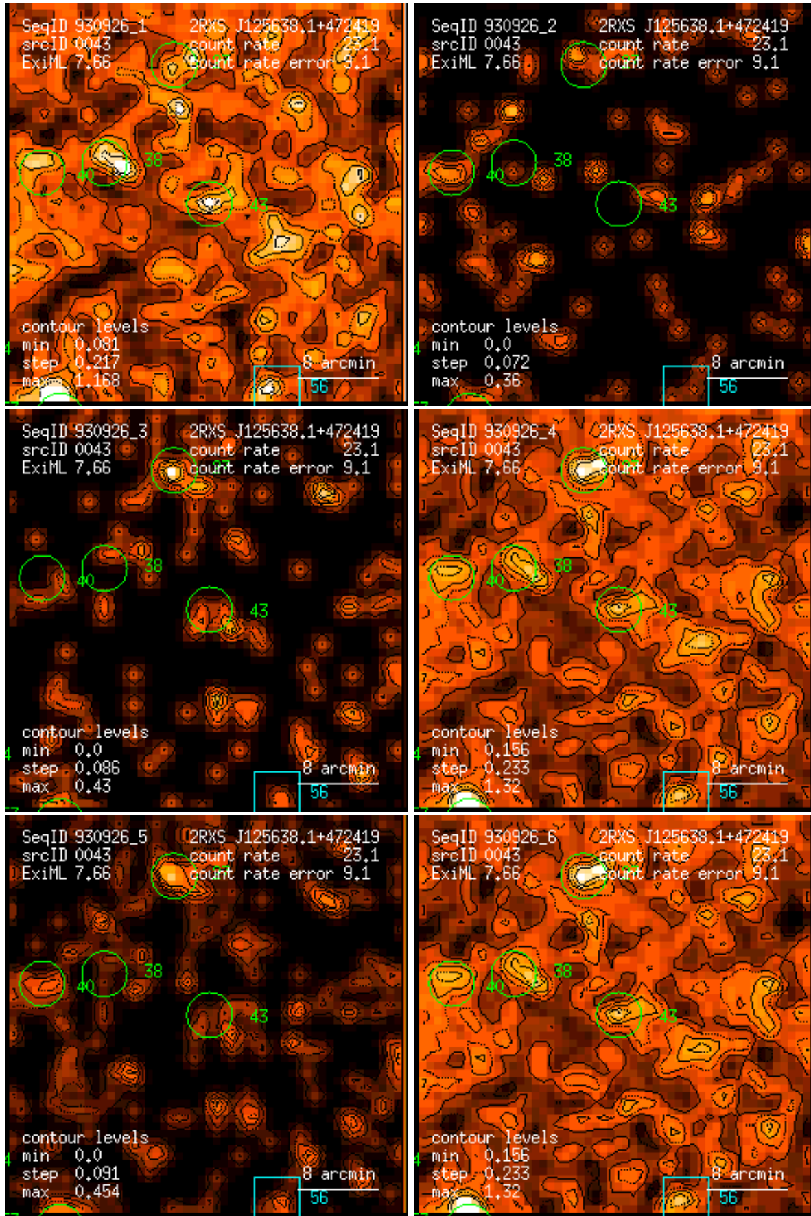
Figure 43: RASS 930926: detection 0043: band rate images, Gaussian filter: (1) PSPC channels 11 – 41, (2) 52 – 90, (3) 91 – 201, (4) 11 – 235, (5) 52 – 201, (6) 11 – 201. Broad band rates in counts/ks. Band rate contour levels in counts/ks/arcmin 2 .
