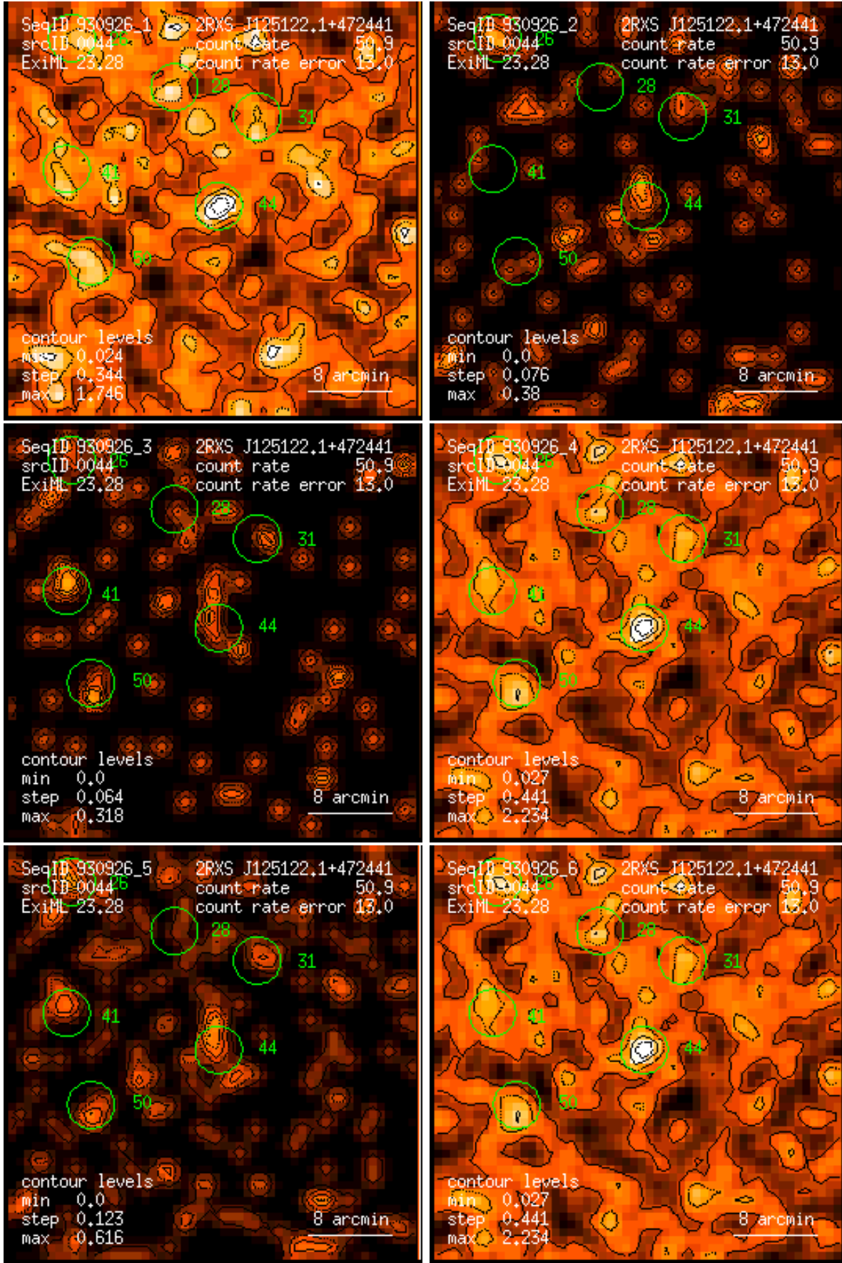
Figure 44: RASS 930926: detection 0044: band rate images, Gaussian filter: (1) PSPC channels 11 – 41, (2) 52 – 90, (3) 91 – 201, (4) 11 – 235, (5) 52 – 201, (6) 11 – 201. Broad band rates in counts/ks. Band rate contour levels in counts/ks/arcmin 2 .
