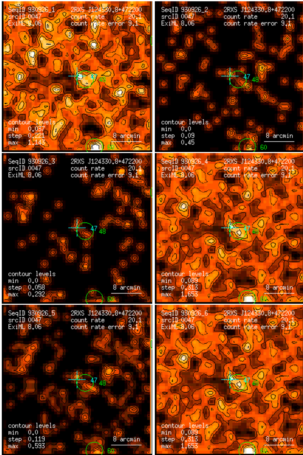
Figure 47: RASS 930926: detection 0047: band rate images, Gaussian filter: (1) PSPC channels 11 – 41, (2) 52 – 90, (3) 91 – 201, (4) 11 – 235, (5) 52 – 201, (6) 11 – 201. Broad band rates in counts/ks. Band rate contour levels in counts/ks/arcmin 2 .
