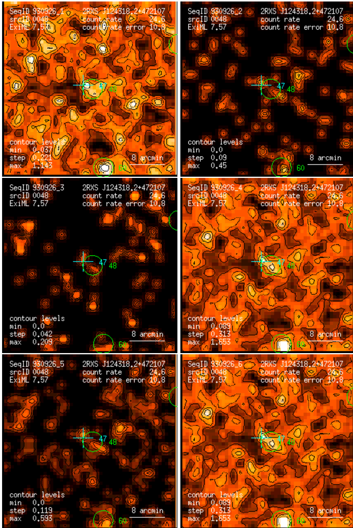
Figure 48: RASS 930926: detection 0048: band rate images, Gaussian filter: (1) PSPC channels 11 – 41, (2) 52 – 90, (3) 91 – 201, (4) 11 – 235, (5) 52 – 201, (6) 11 – 201. Broad band rates in counts/ks. Band rate contour levels in counts/ks/arcmin 2 .
