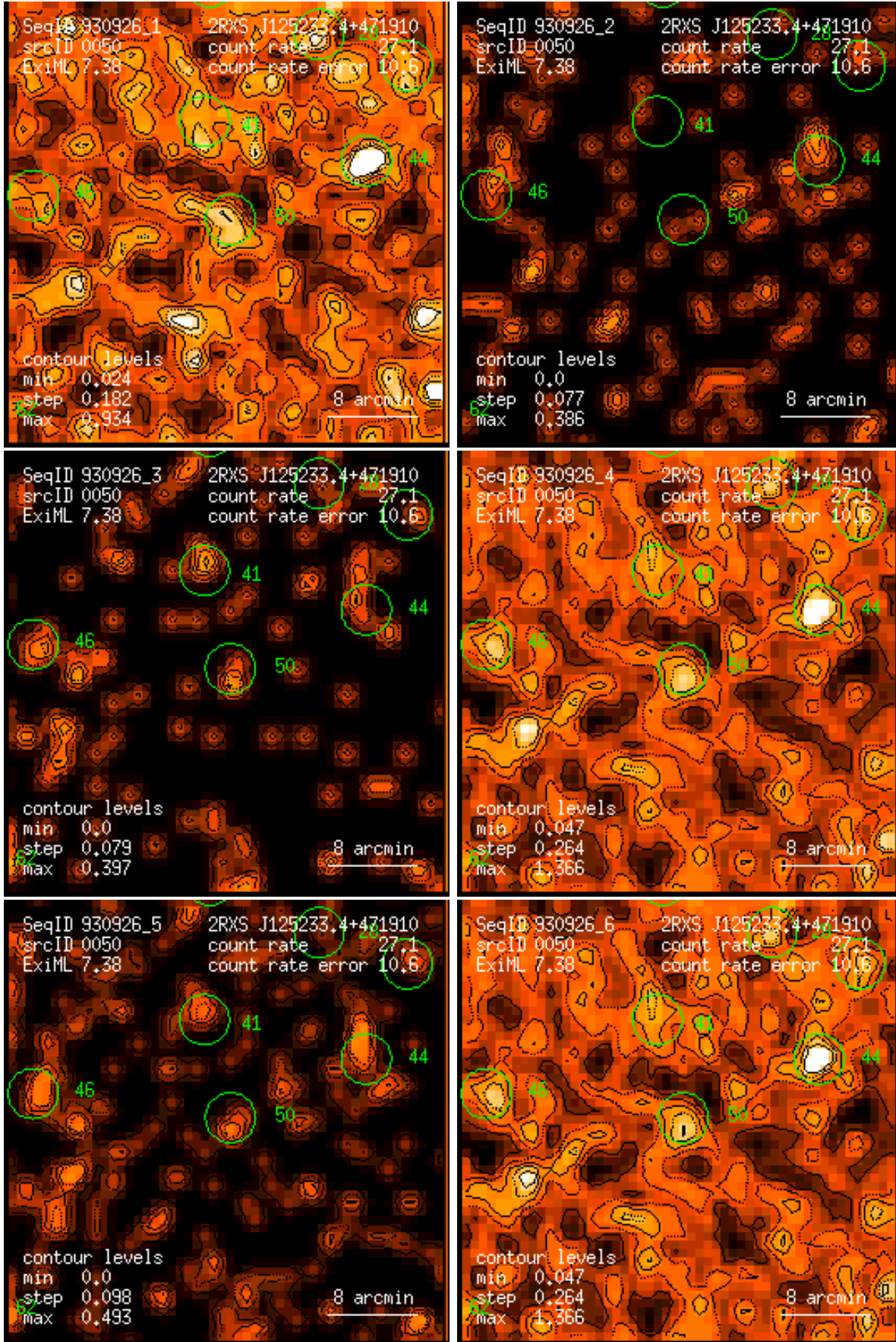
Figure 50: RASS 930926: detection 0050: band rate images, Gaussian filter: (1) PSPC channels 11 – 41, (2) 52 – 90, (3) 91 – 201, (4) 11 – 235, (5) 52 – 201, (6) 11 – 201. Broad band rates in counts/ks. Band rate contour levels in counts/ks/arcmin 2 .
