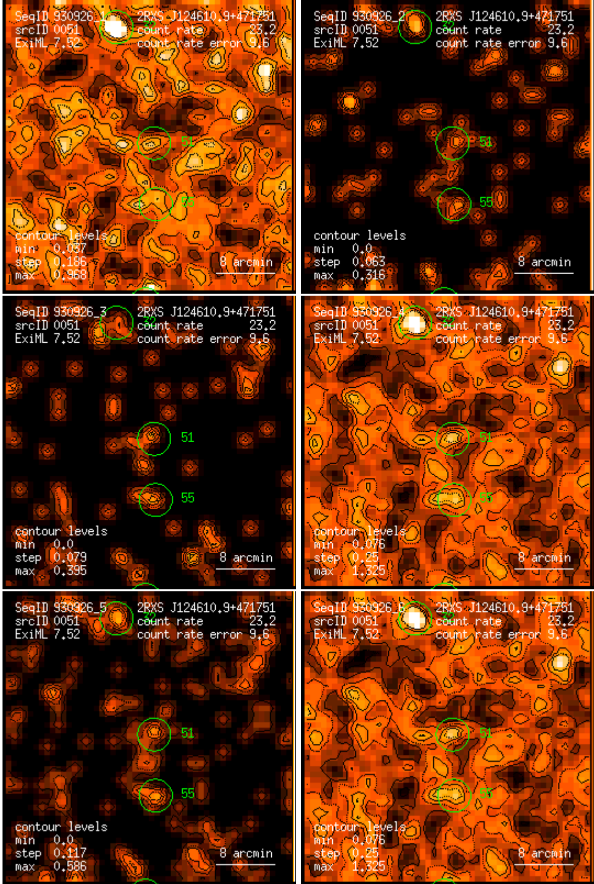
Figure 51: RASS 930926: detection 0051: band rate images, Gaussian filter: (1) PSPC channels 11 – 41, (2) 52 – 90, (3) 91 – 201, (4) 11 – 235, (5) 52 – 201, (6) 11 – 201. Broad band rates in counts/ks. Band rate contour levels in counts/ks/arcmin 2 .
