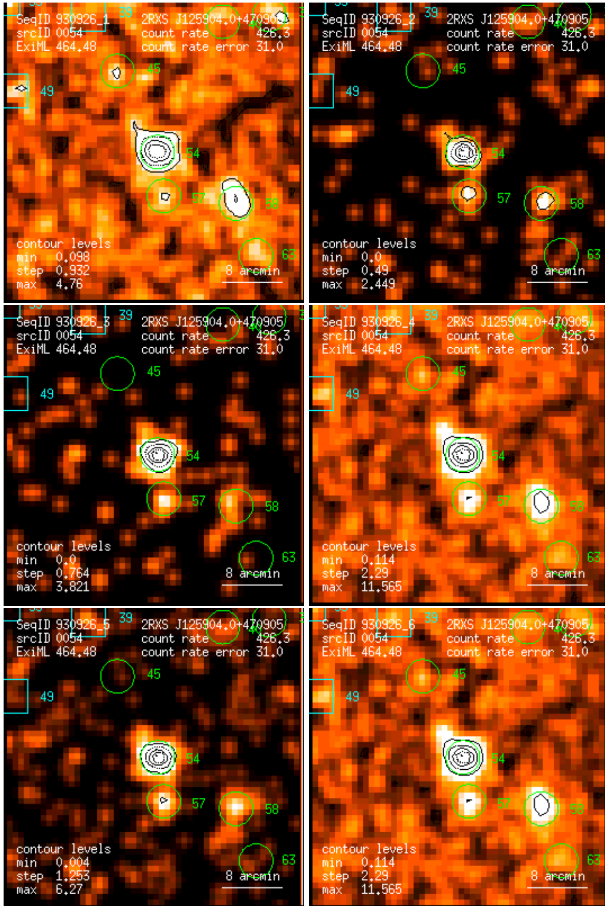
Figure 54: RASS 930926: detection 0054: band rate images, Gaussian filter: (1) PSPC channels 11 – 41, (2) 52 – 90, (3) 91 – 201, (4) 11 – 235, (5) 52 – 201, (6) 11 – 201. Broad band rates in counts/ks. Band rate contour levels in counts/ks/arcmin 2 .
