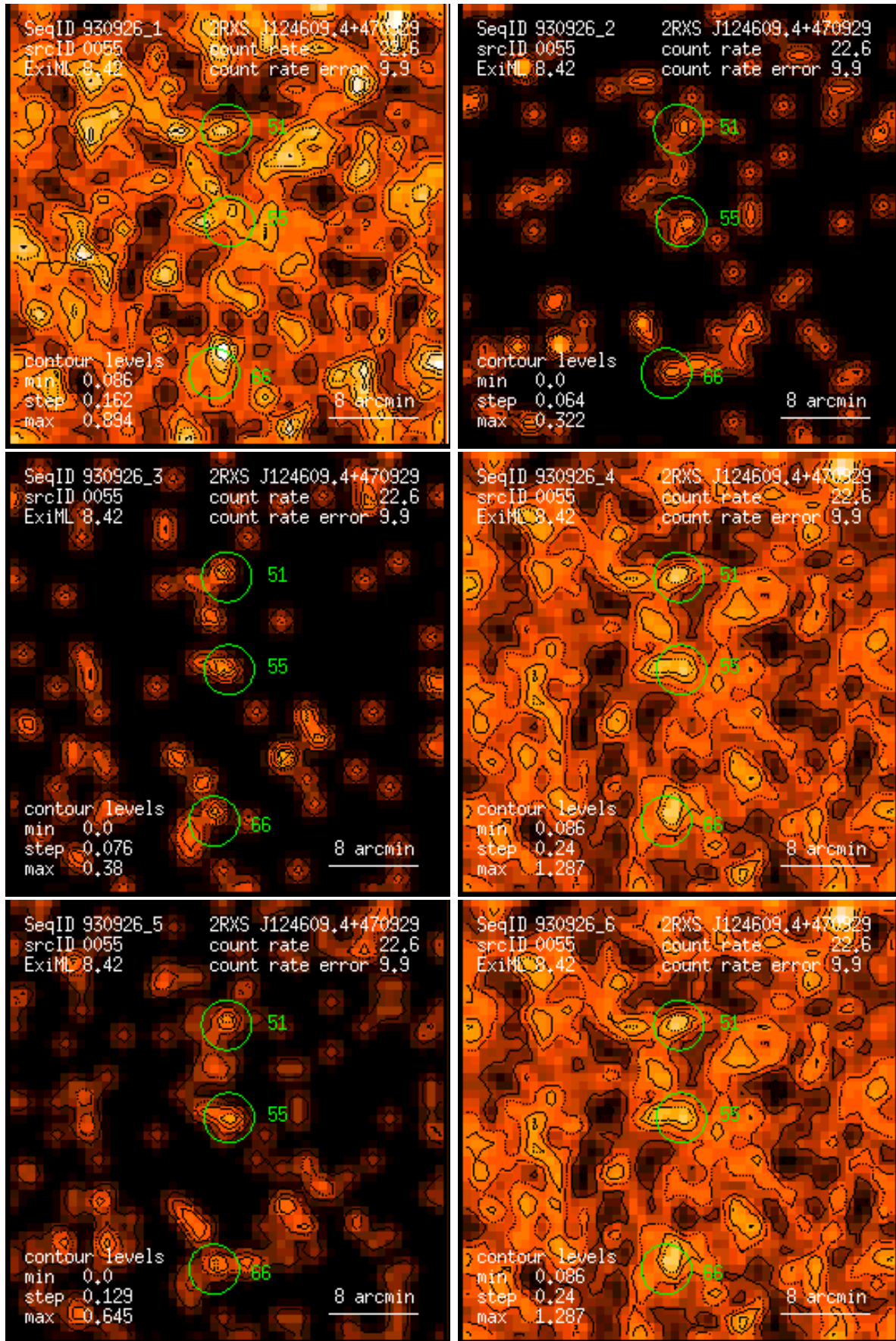
Figure 55: RASS 930926: detection 0055: band rate images, Gaussian filter: (1) PSPC channels 11 – 41, (2) 52 – 90, (3) 91 – 201, (4) 11 – 235, (5) 52 – 201, (6) 11 – 201. Broad band rates in counts/ks. Band rate contour levels in counts/ks/arcmin 2 .
