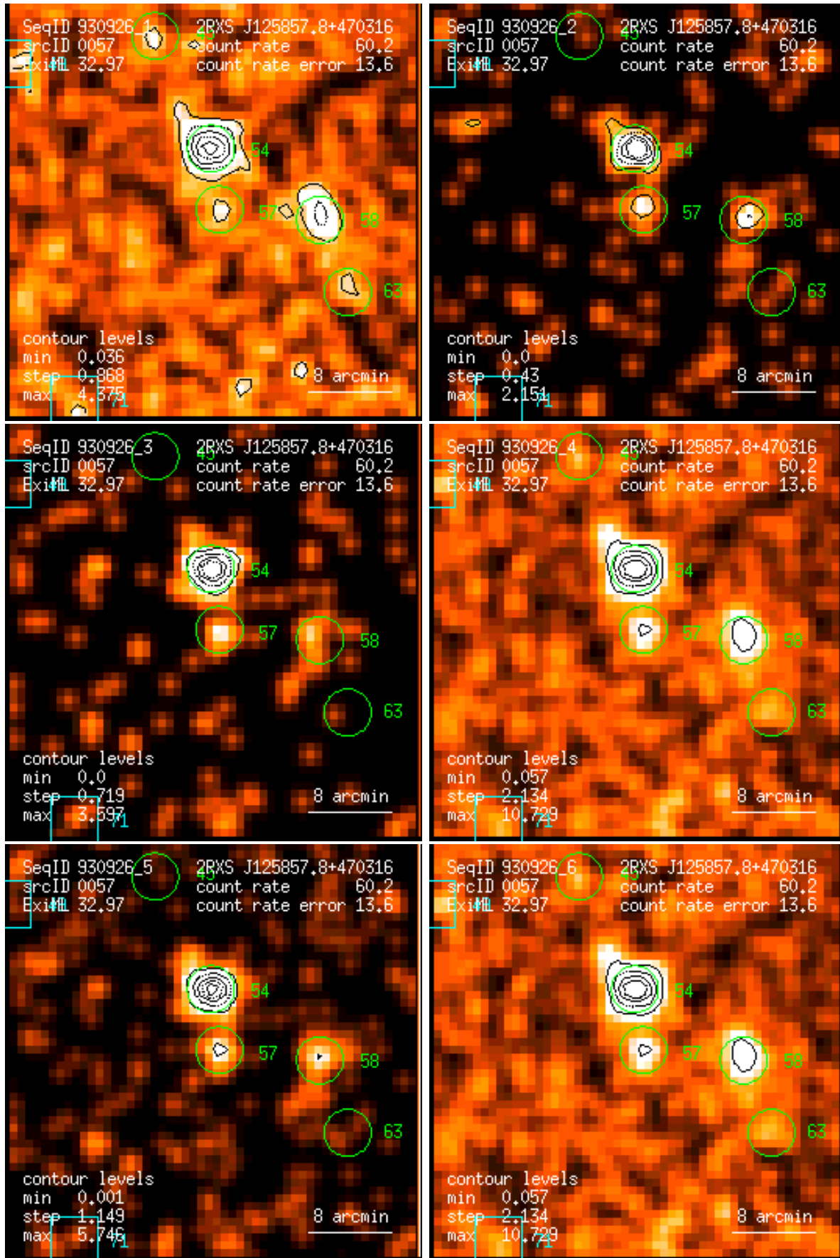
Figure 57: RASS 930926: detection 0057: band rate images, Gaussian filter: (1) PSPC channels 11 – 41, (2) 52 – 90, (3) 91 – 201, (4) 11 – 235, (5) 52 – 201, (6) 11 – 201. Broad band rates in counts/ks. Band rate contour levels in counts/ks/arcmin 2 .
