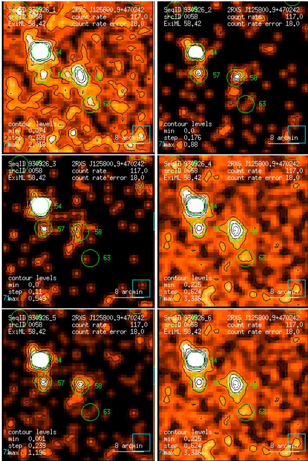
Figure 58: RASS 930926: detection 0058: band rate images, Gaussian filter: (1) PSPC channels 11 – 41, (2) 52 – 90, (3) 91 – 201, (4) 11 – 235, (5) 52 – 201, (6) 11 – 201. Broad band rates in counts/ks. Band rate contour levels in counts/ks/arcmin 2 .
