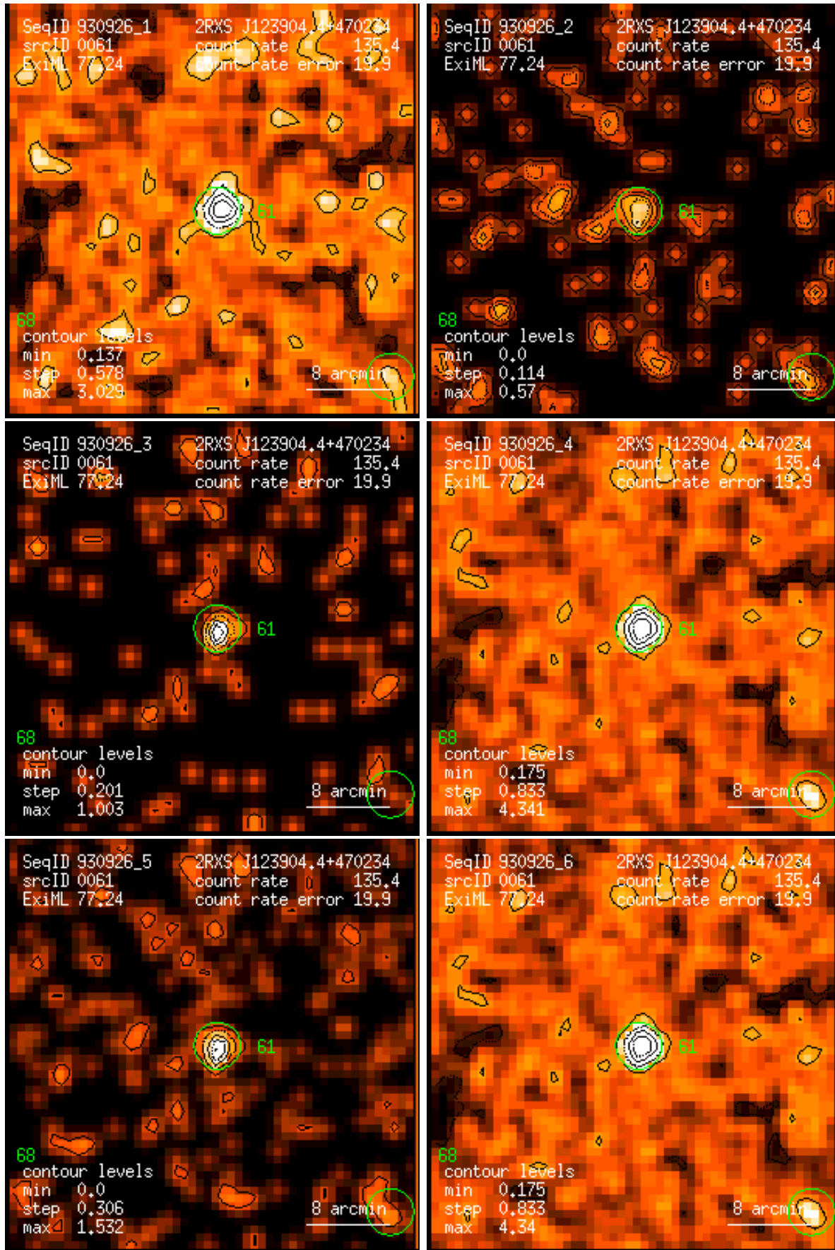
Figure 61: RASS 930926: detection 0061: band rate images, Gaussian filter: (1) PSPC channels 11 – 41, (2) 52 – 90, (3) 91 – 201, (4) 11 – 235, (5) 52 – 201, (6) 11 – 201. Broad band rates in counts/ks. Band rate contour levels in counts/ks/arcmin 2 .
