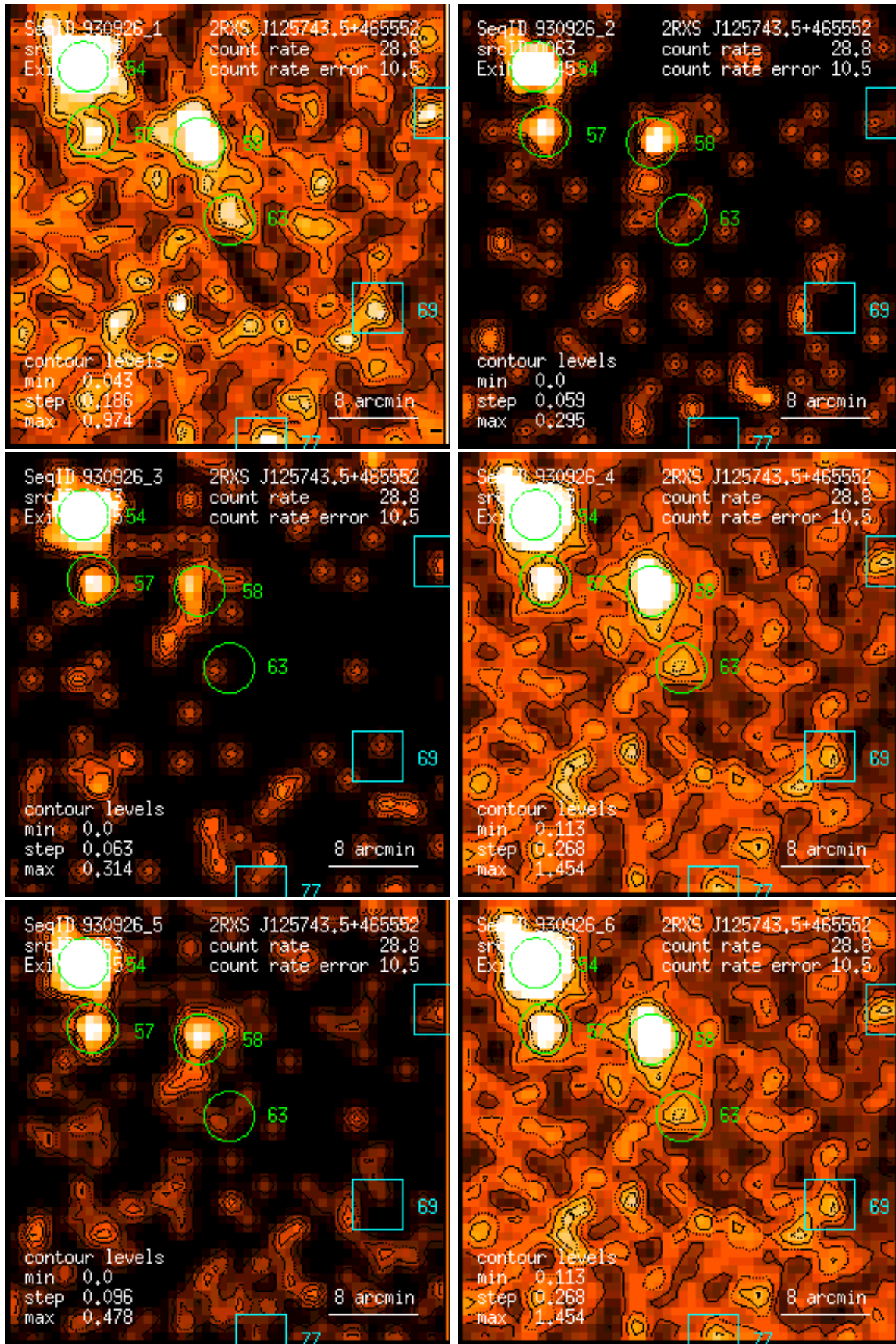
Figure 63: RASS 930926: detection 0063: band rate images, Gaussian filter: (1) PSPC channels 11 – 41, (2) 52 – 90, (3) 91 – 201, (4) 11 – 235, (5) 52 – 201, (6) 11 – 201. Broad band rates in counts/ks. Band rate contour levels in counts/ks/arcmin 2 .
