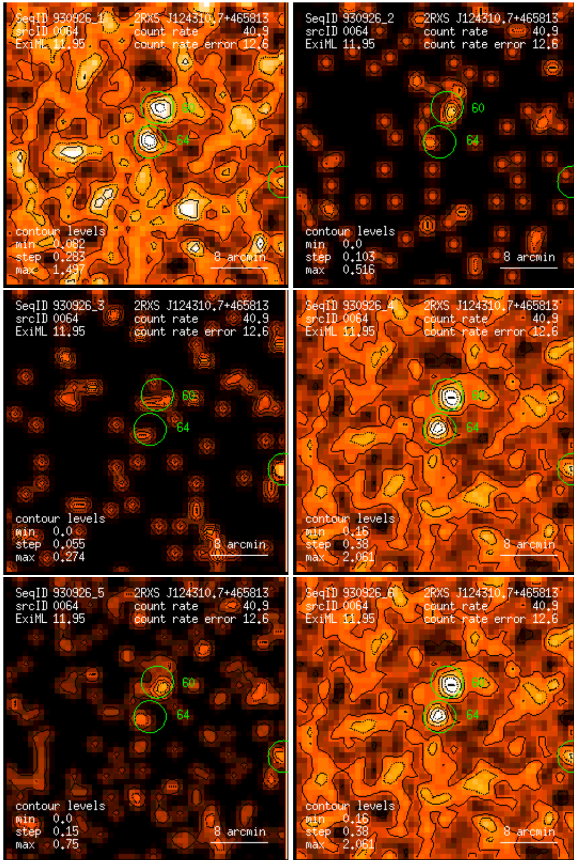
Figure 64: RASS 930926: detection 0064: band rate images, Gaussian filter: (1) PSPC channels 11 – 41, (2) 52 – 90, (3) 91 – 201, (4) 11 – 235, (5) 52 – 201, (6) 11 – 201. Broad band rates in counts/ks. Band rate contour levels in counts/ks/arcmin 2 .
