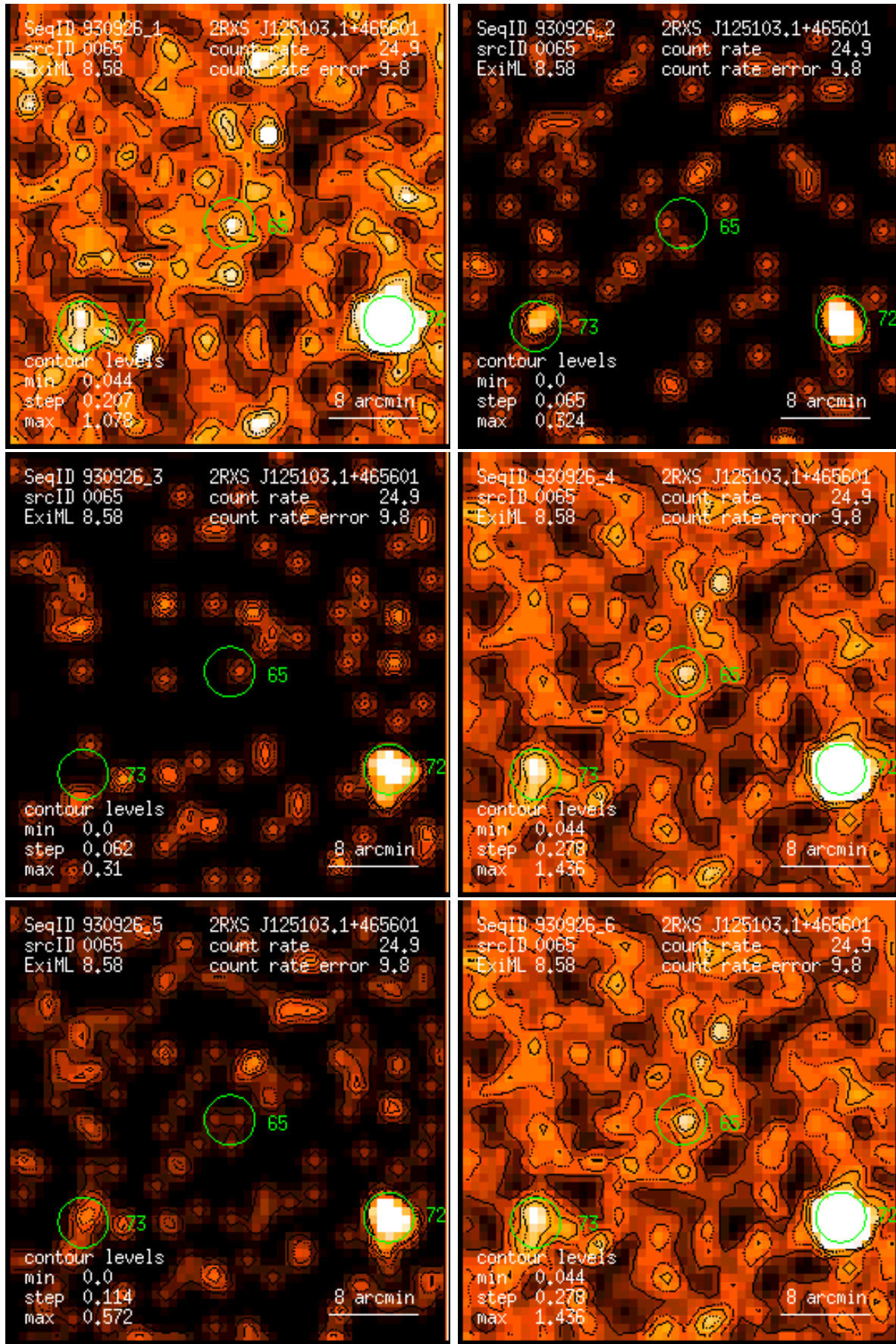
Figure 65: RASS 930926: detection 0065: band rate images, Gaussian filter: (1) PSPC channels 11 – 41, (2) 52 – 90, (3) 91 – 201, (4) 11 – 235, (5) 52 – 201, (6) 11 – 201. Broad band rates in counts/ks. Band rate contour levels in counts/ks/arcmin 2 .
