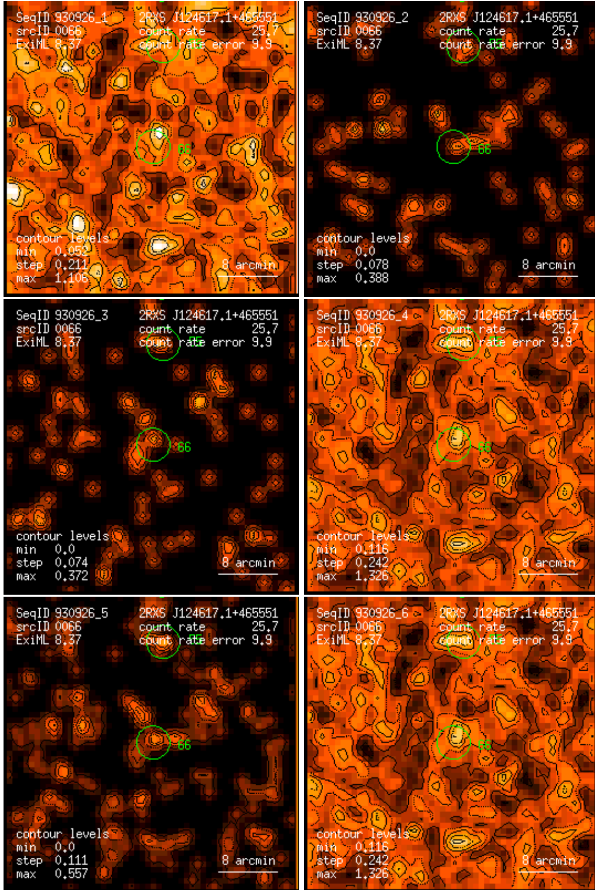
Figure 66: RASS 930926: detection 0066: band rate images, Gaussian filter: (1) PSPC channels 11 – 41, (2) 52 – 90, (3) 91 – 201, (4) 11 – 235, (5) 52 – 201, (6) 11 – 201. Broad band rates in counts/ks. Band rate contour levels in counts/ks/arcmin 2 .
