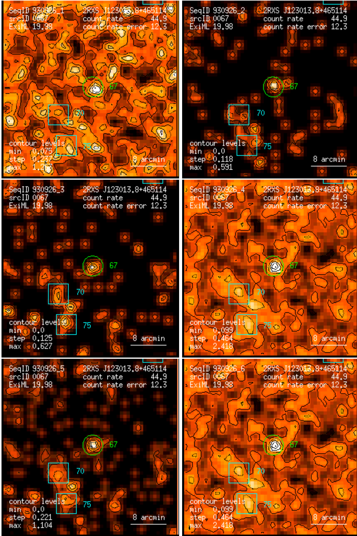
Figure 67: RASS 930926: detection 0067: band rate images, Gaussian filter: (1) PSPC channels 11 – 41, (2) 52 – 90, (3) 91 – 201, (4) 11 – 235, (5) 52 – 201, (6) 11 – 201. Broad band rates in counts/ks. Band rate contour levels in counts/ks/arcmin 2 .
