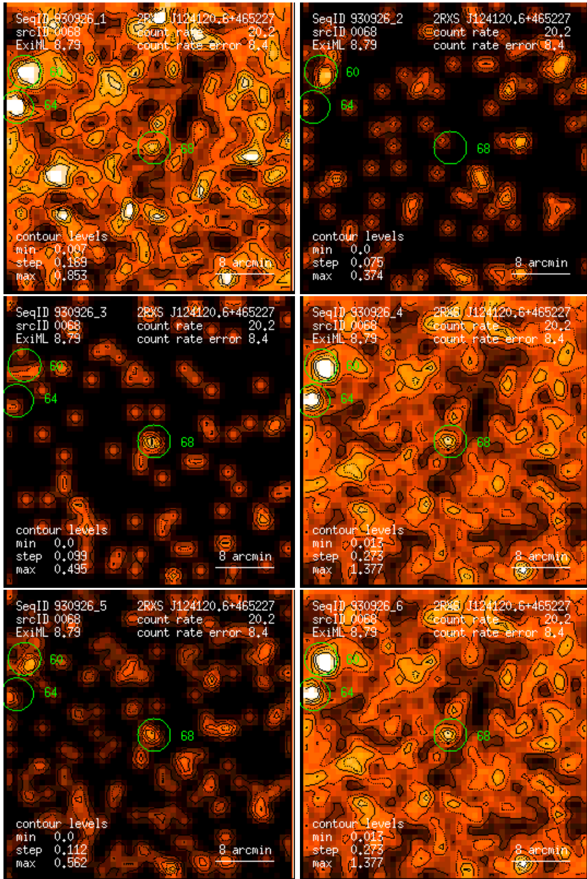
Figure 68: RASS 930926: detection 0068: band rate images, Gaussian filter: (1) PSPC channels 11 – 41, (2) 52 – 90, (3) 91 – 201, (4) 11 – 235, (5) 52 – 201, (6) 11 – 201. Broad band rates in counts/ks. Band rate contour levels in counts/ks/arcmin 2 .
