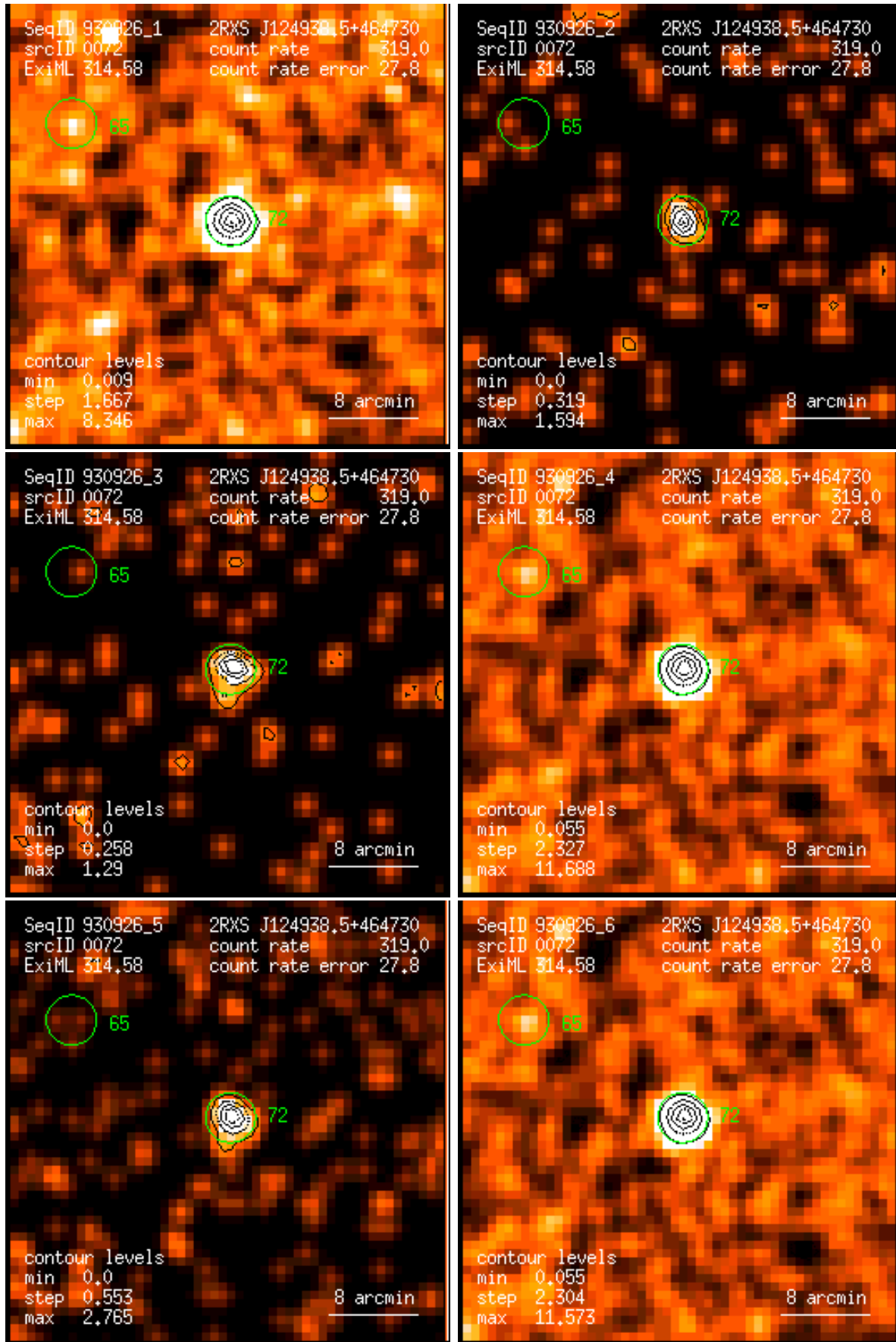
Figure 72: RASS 930926: detection 0072: band rate images, Gaussian filter: (1) PSPC channels 11 – 41, (2) 52 – 90, (3) 91 – 201, (4) 11 – 235, (5) 52 – 201, (6) 11 – 201. Broad band rates in counts/ks. Band rate contour levels in counts/ks/arcmin 2 .
