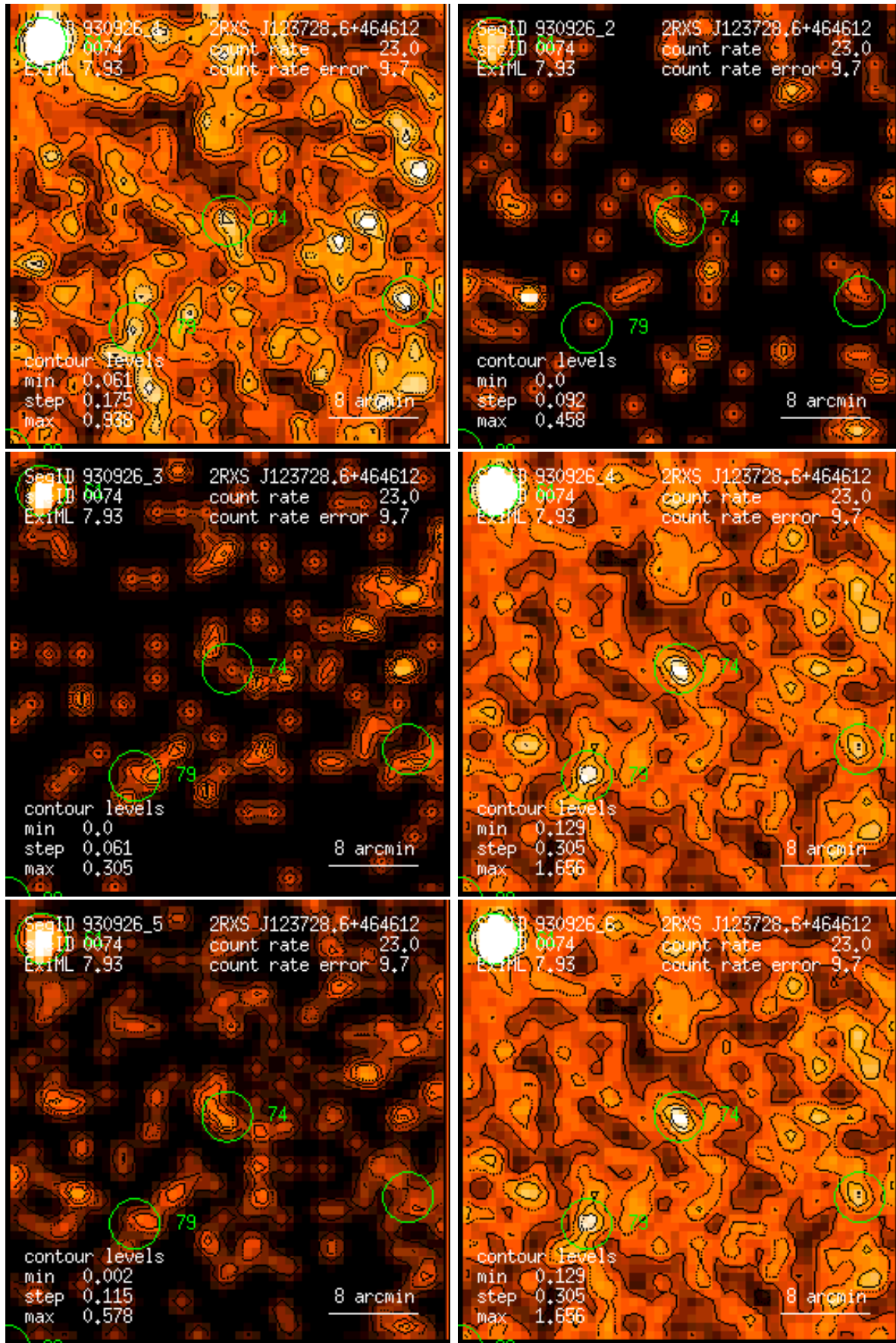
Figure 74: RASS 930926: detection 0074: band rate images, Gaussian filter: (1) PSPC channels 11 – 41, (2) 52 – 90, (3) 91 – 201, (4) 11 – 235, (5) 52 – 201, (6) 11 – 201. Broad band rates in counts/ks. Band rate contour levels in counts/ks/arcmin 2 .
