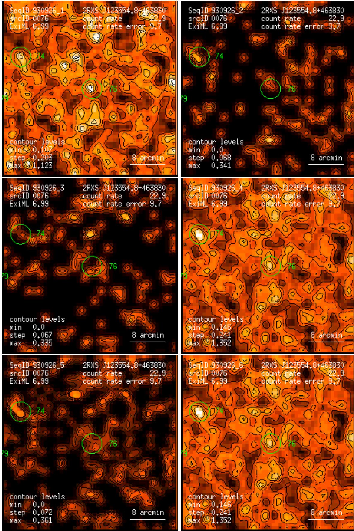
Figure 76: RASS 930926: detection 0076: band rate images, Gaussian filter: (1) PSPC channels 11 – 41, (2) 52 – 90, (3) 91 – 201, (4) 11 – 235, (5) 52 – 201, (6) 11 – 201. Broad band rates in counts/ks. Band rate contour levels in counts/ks/arcmin 2 .
