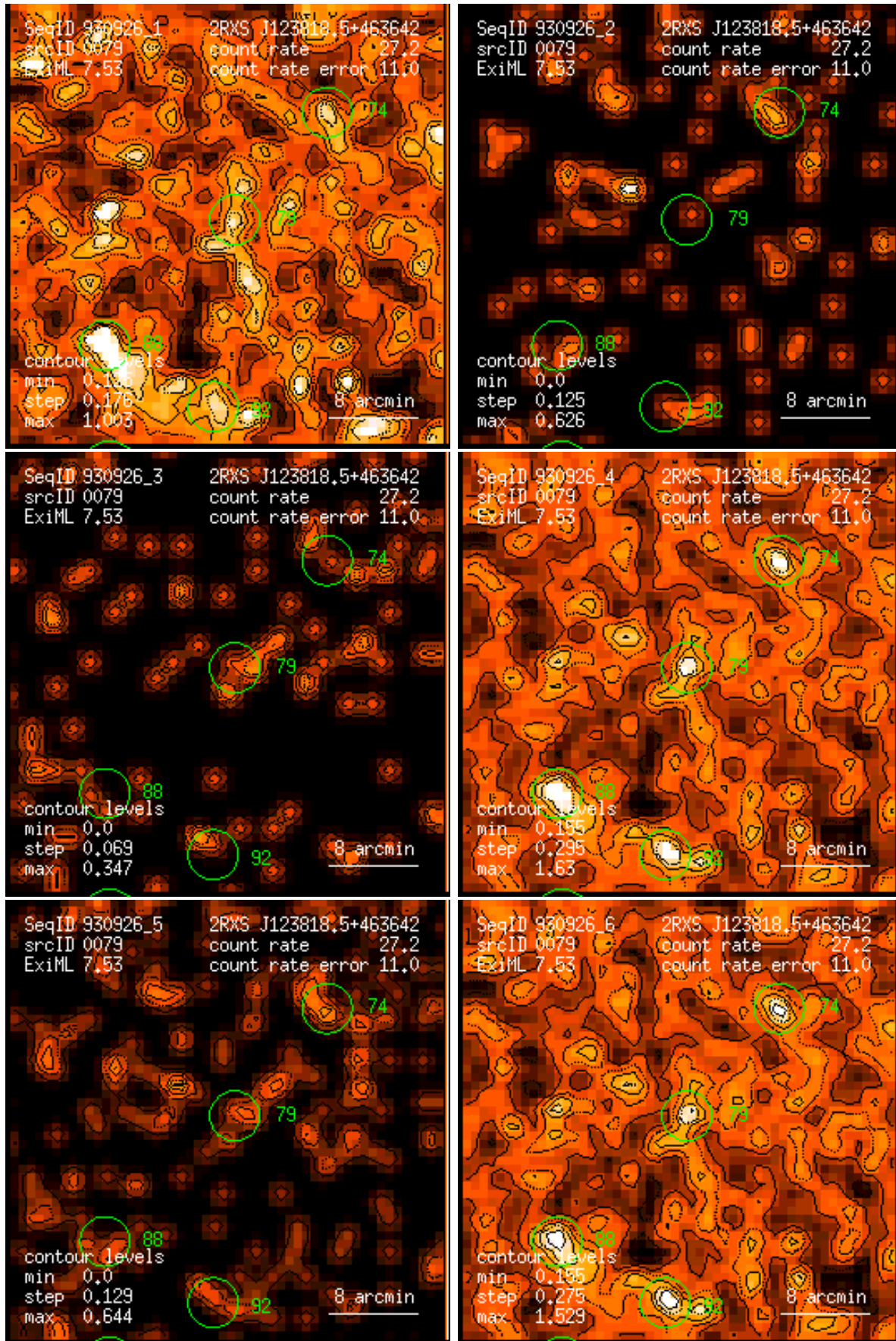
Figure 79: RASS 930926: detection 0079: band rate images, Gaussian filter: (1) PSPC channels 11 – 41, (2) 52 – 90, (3) 91 – 201, (4) 11 – 235, (5) 52 – 201, (6) 11 – 201. Broad band rates in counts/ks. Band rate contour levels in counts/ks/arcmin 2 .
