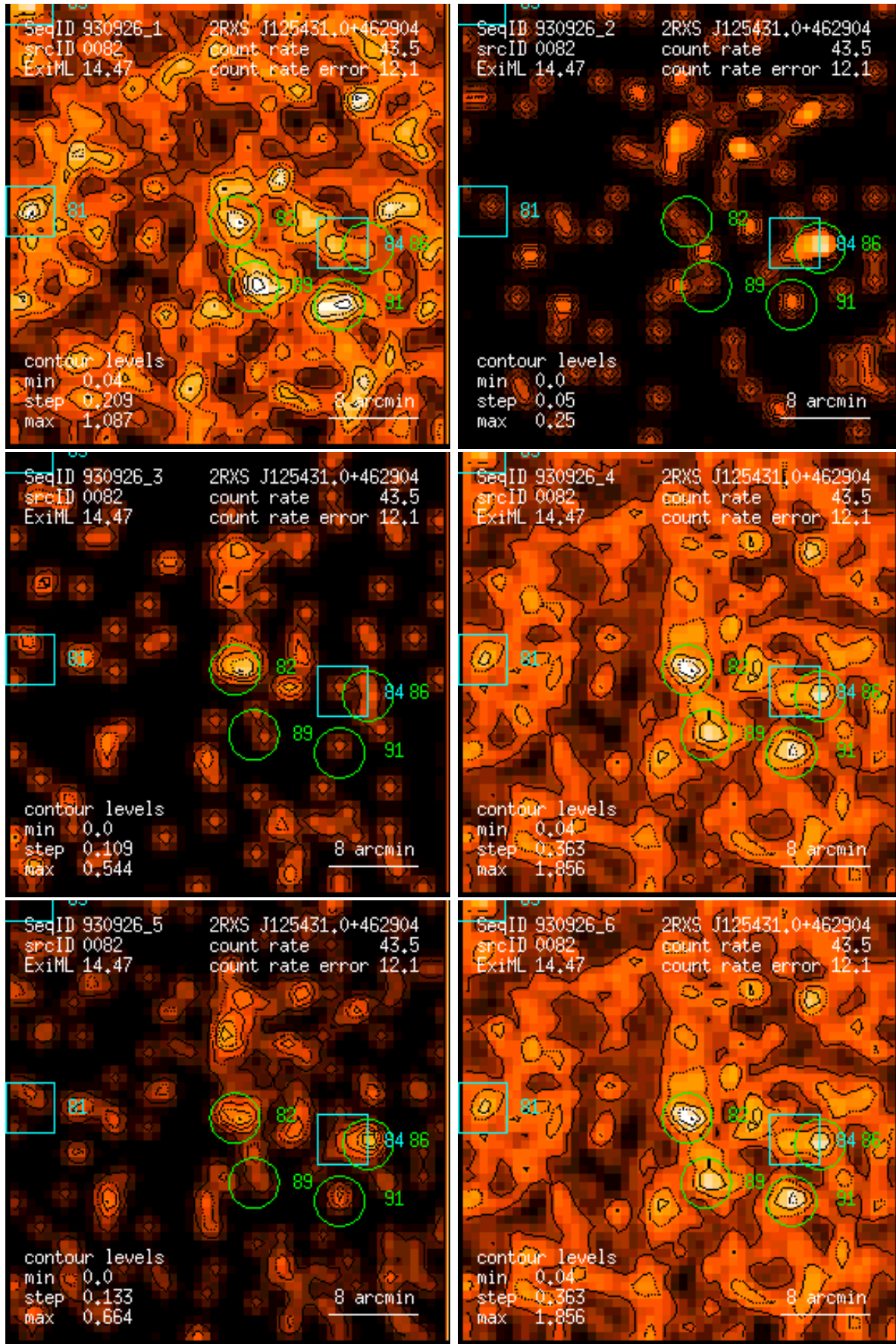
Figure 82: RASS 930926: detection 0082: band rate images, Gaussian filter: (1) PSPC channels 11 – 41, (2) 52 – 90, (3) 91 – 201, (4) 11 – 235, (5) 52 – 201, (6) 11 – 201. Broad band rates in counts/ks. Band rate contour levels in counts/ks/arcmin 2 .
