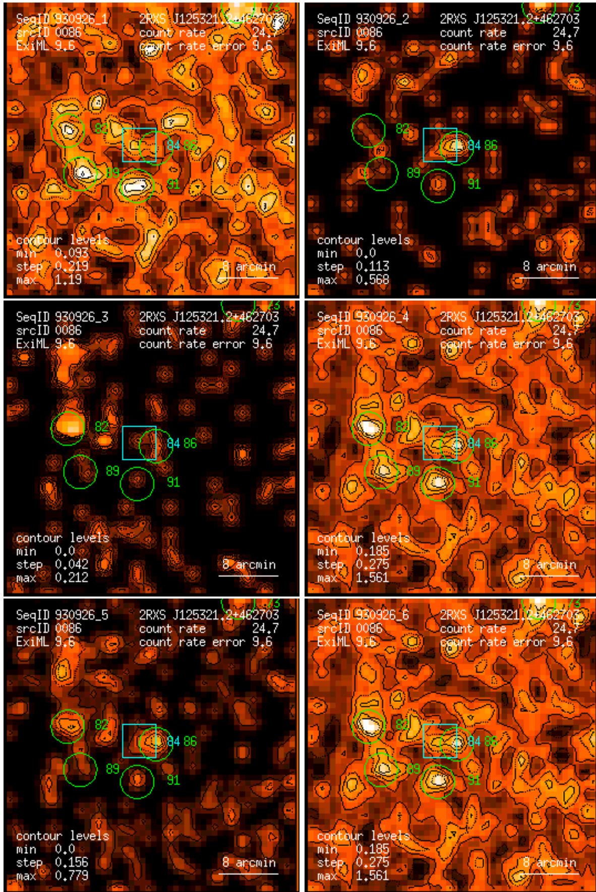
Figure 86: RASS 930926: detection 0086: band rate images, Gaussian filter: (1) PSPC channels 11 – 41, (2) 52 – 90, (3) 91 – 201, (4) 11 – 235, (5) 52 – 201, (6) 11 – 201. Broad band rates in counts/ks. Band rate contour levels in counts/ks/arcmin 2 .
