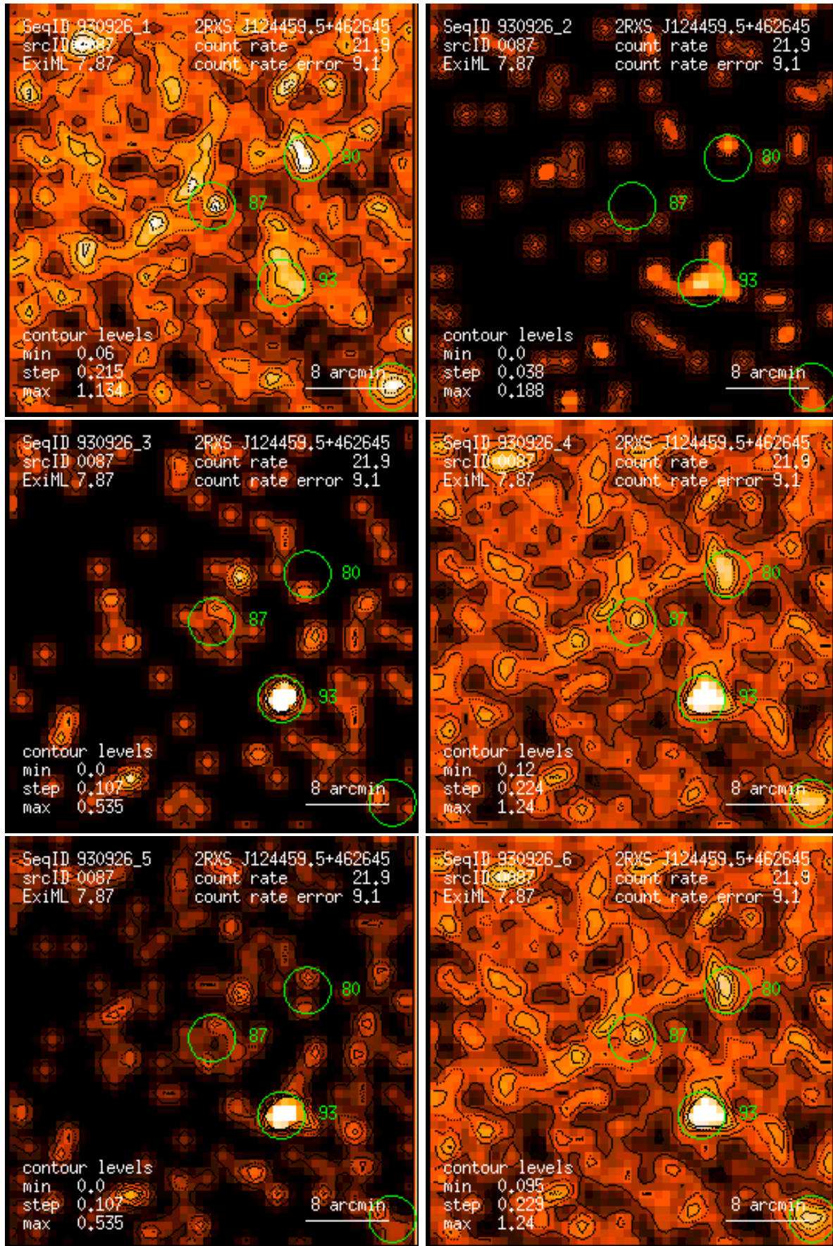
Figure 87: RASS 930926: detection 0087: band rate images, Gaussian filter: (1) PSPC channels 11 – 41, (2) 52 – 90, (3) 91 – 201, (4) 11 – 235, (5) 52 – 201, (6) 11 – 201. Broad band rates in counts/ks. Band rate contour levels in counts/ks/arcmin 2 .
