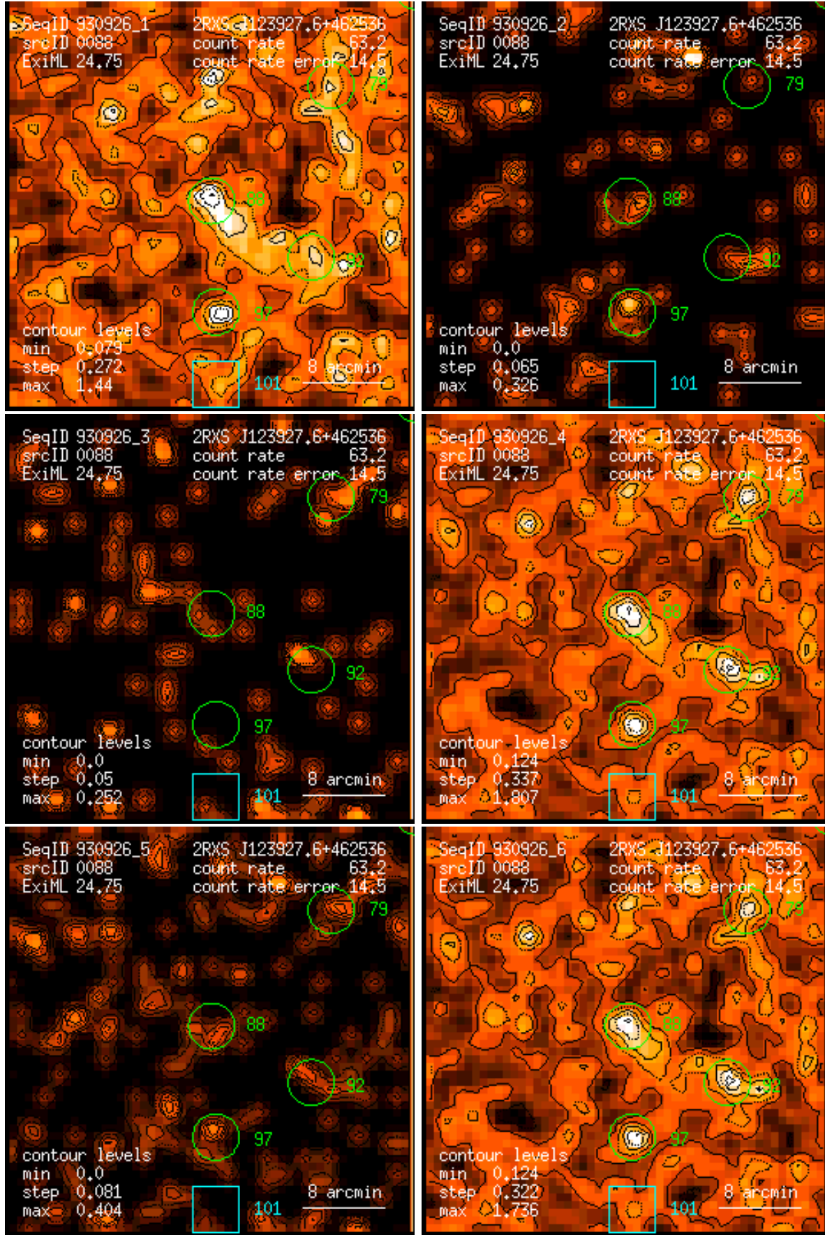
Figure 88: RASS 930926: detection 0088: band rate images, Gaussian filter: (1) PSPC channels 11 – 41, (2) 52 – 90, (3) 91 – 201, (4) 11 – 235, (5) 52 – 201, (6) 11 – 201. Broad band rates in counts/ks. Band rate contour levels in counts/ks/arcmin 2 .
