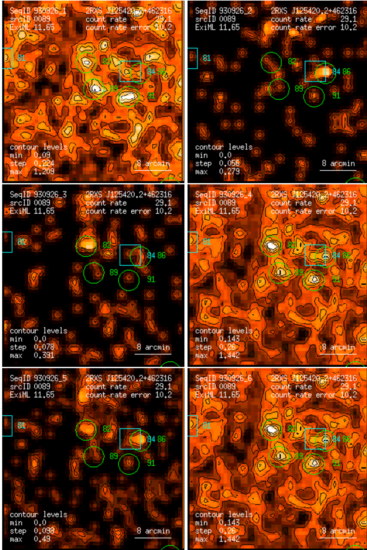
Figure 89: RASS 930926: detection 0089: band rate images, Gaussian filter: (1) PSPC channels 11 – 41, (2) 52 – 90, (3) 91 – 201, (4) 11 – 235, (5) 52 – 201, (6) 11 – 201. Broad band rates in counts/ks. Band rate contour levels in counts/ks/arcmin 2 .
