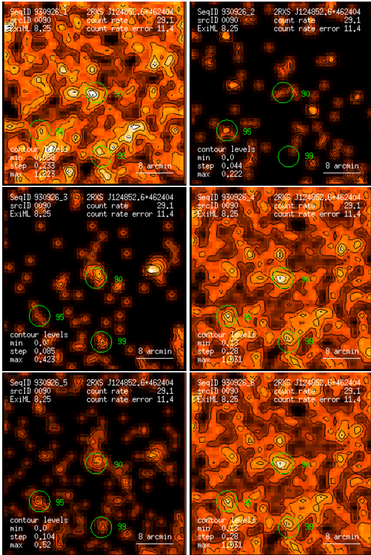
Figure 90: RASS 930926: detection 0090: band rate images, Gaussian filter: (1) PSPC channels 11 – 41, (2) 52 – 90, (3) 91 – 201, (4) 11 – 235, (5) 52 – 201, (6) 11 – 201. Broad band rates in counts/ks. Band rate contour levels in counts/ks/arcmin 2 .
