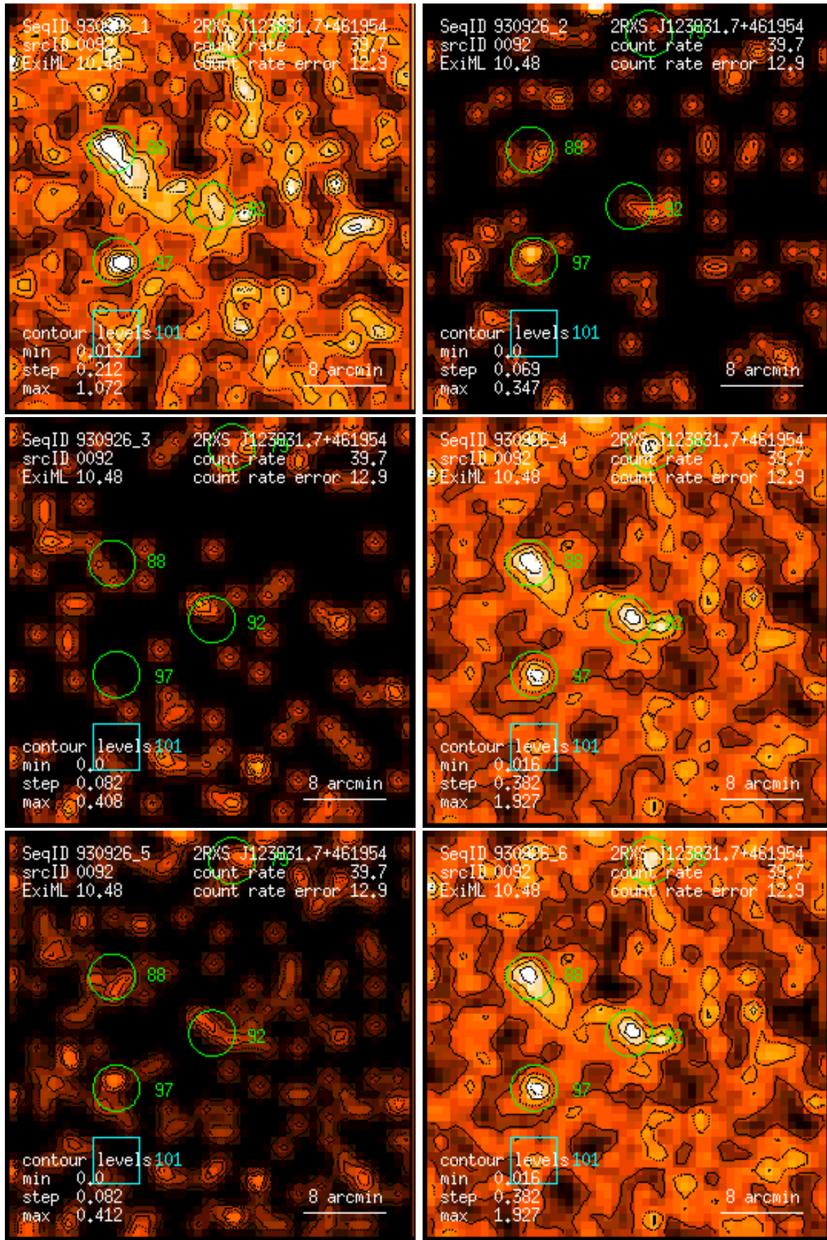
Figure 92: RASS 930926: detection 0092: band rate images, Gaussian filter: (1) PSPC channels 11 – 41, (2) 52 – 90, (3) 91 – 201, (4) 11 – 235, (5) 52 – 201, (6) 11 – 201. Broad band rates in counts/ks. Band rate contour levels in counts/ks/arcmin 2 .
