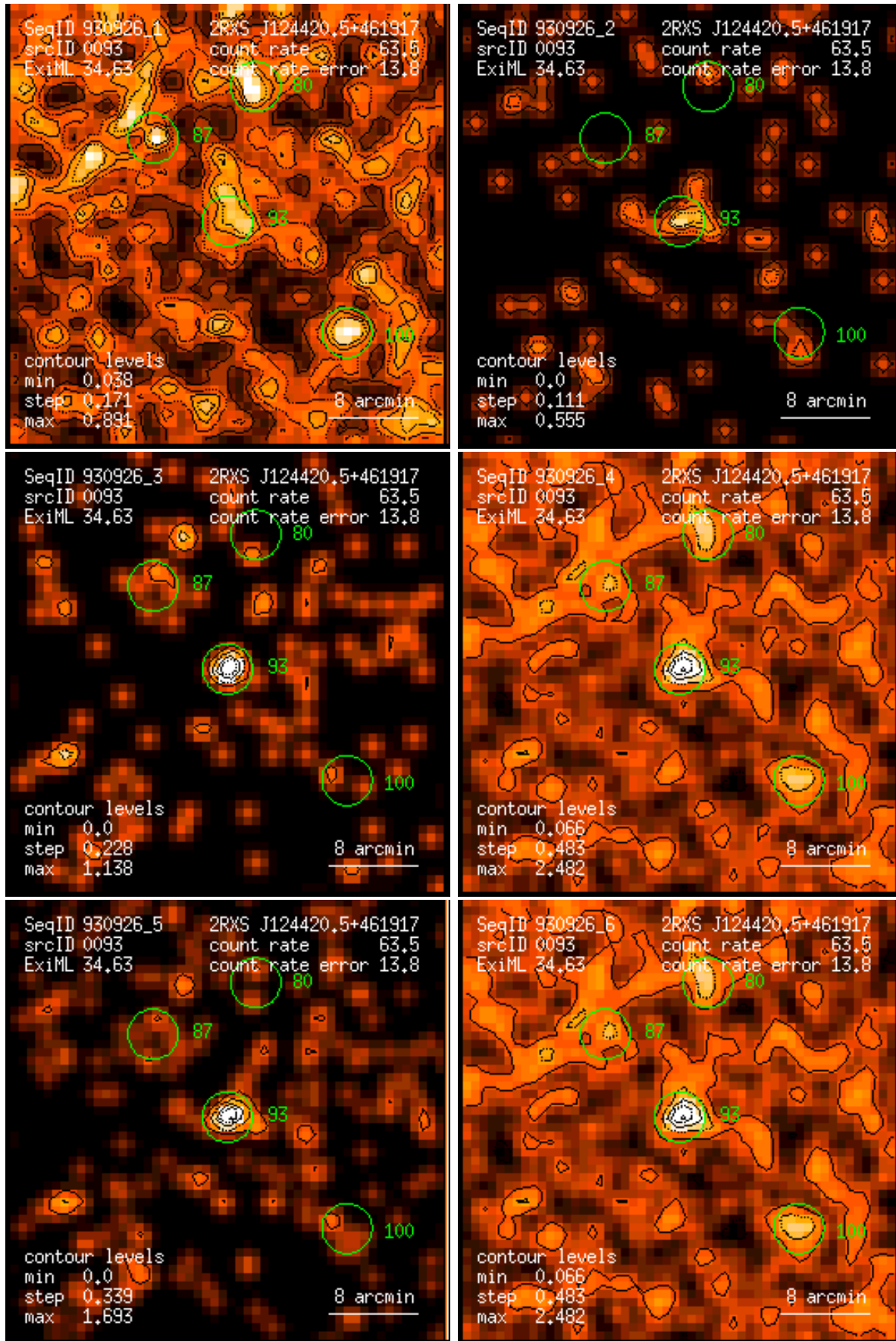
Figure 93: RASS 930926: detection 0093: band rate images, Gaussian filter: (1) PSPC channels 11 – 41, (2) 52 – 90, (3) 91 – 201, (4) 11 – 235, (5) 52 – 201, (6) 11 – 201. Broad band rates in counts/ks. Band rate contour levels in counts/ks/arcmin 2 .
