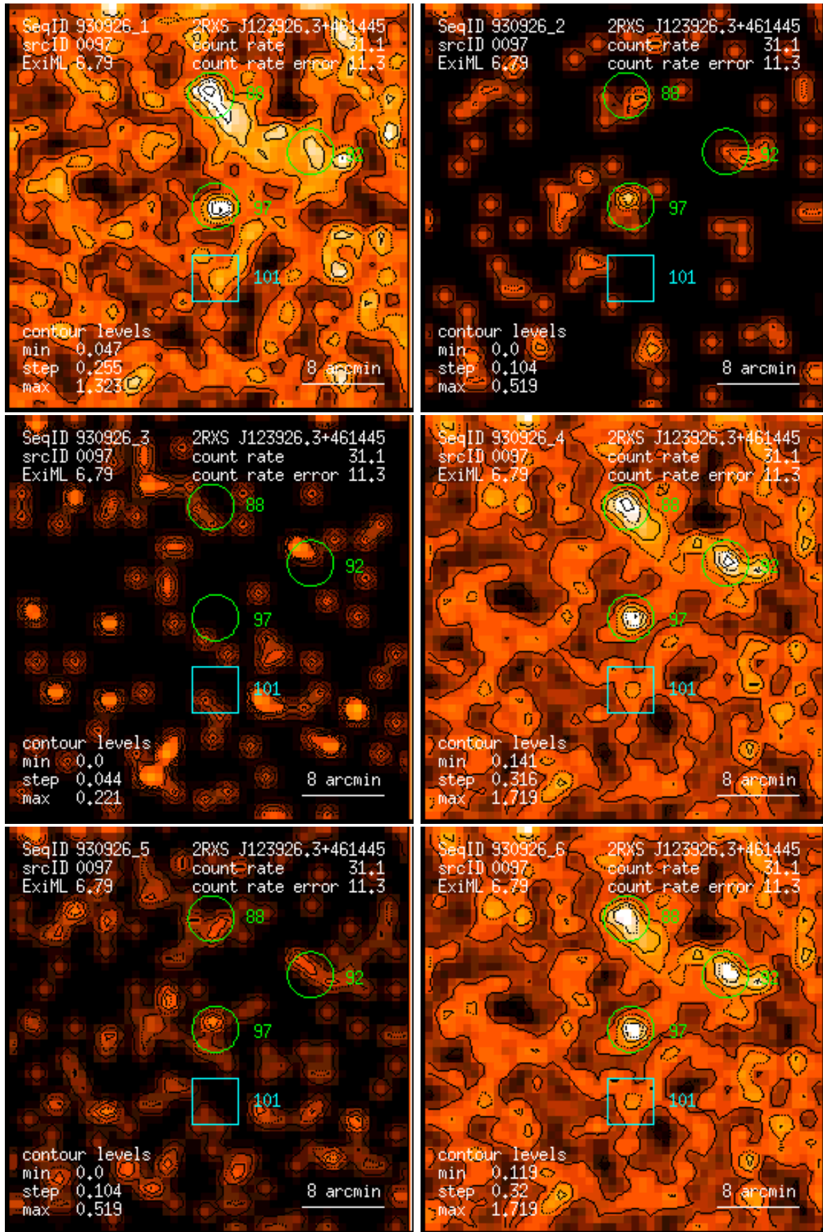
Figure 97: RASS 930926: detection 0097: band rate images, Gaussian filter: (1) PSPC channels 11 – 41, (2) 52 – 90, (3) 91 – 201, (4) 11 – 235, (5) 52 – 201, (6) 11 – 201. Broad band rates in counts/ks. Band rate contour levels in counts/ks/arcmin 2 .
