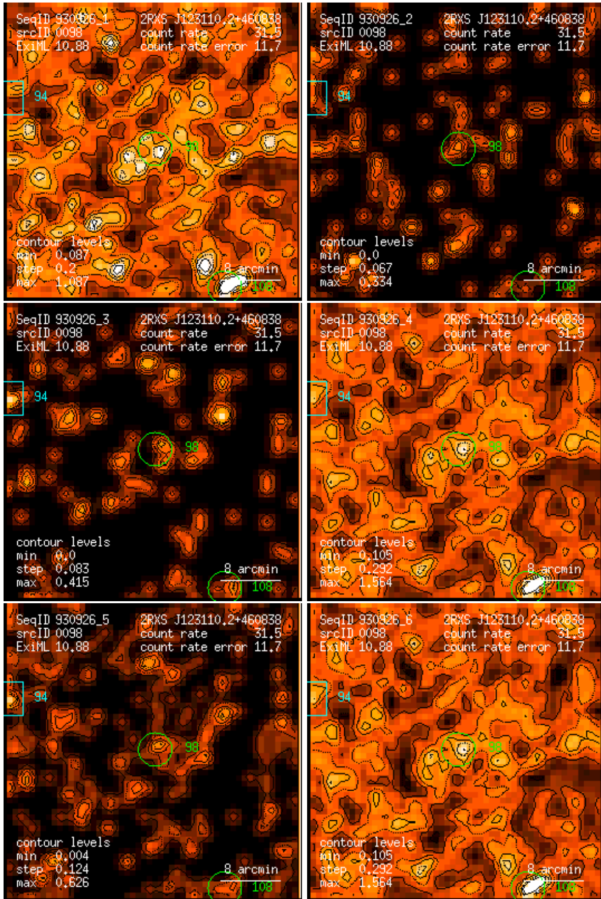
Figure 98: RASS 930926: detection 0098: band rate images, Gaussian filter: (1) PSPC channels 11 – 41, (2) 52 – 90, (3) 91 – 201, (4) 11 – 235, (5) 52 – 201, (6) 11 – 201. Broad band rates in counts/ks. Band rate contour levels in counts/ks/arcmin 2 .
