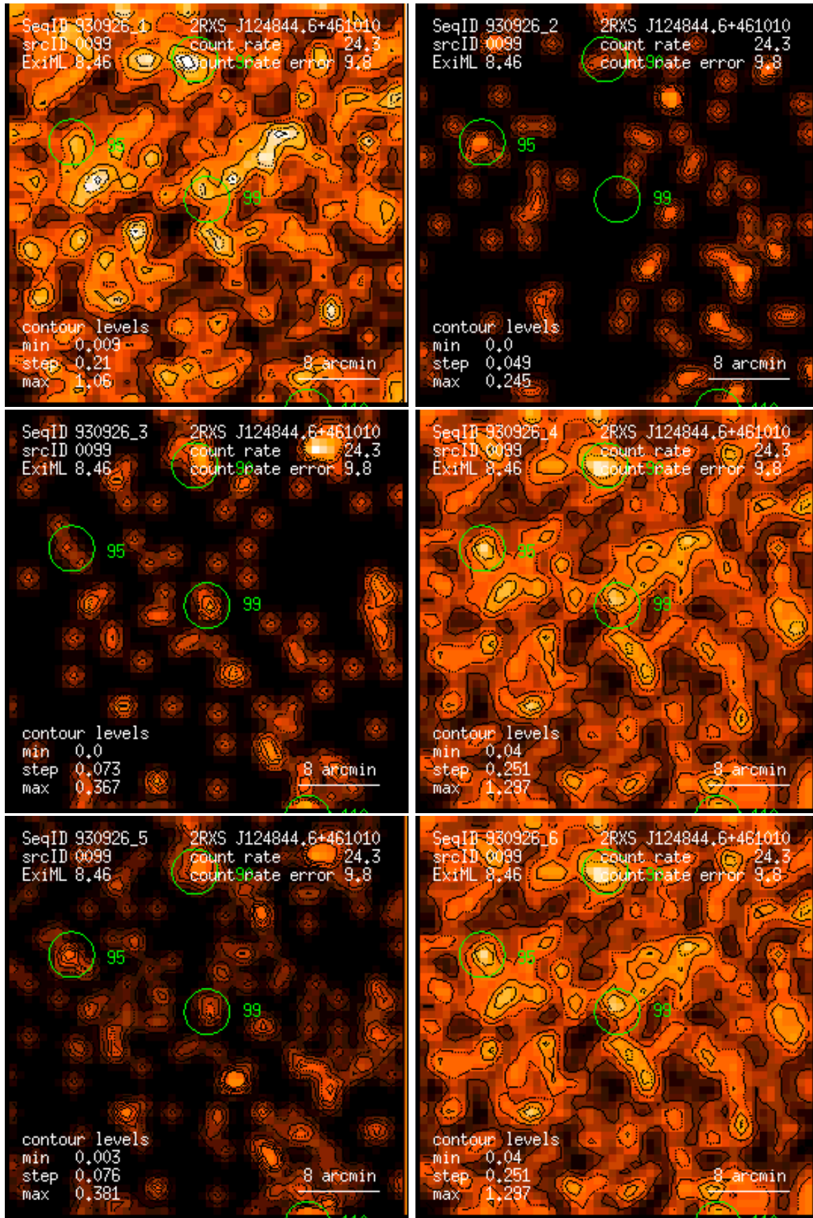
Figure 99: RASS 930926: detection 0099: band rate images, Gaussian filter: (1) PSPC channels 11 – 41, (2) 52 – 90, (3) 91 – 201, (4) 11 – 235, (5) 52 – 201, (6) 11 – 201. Broad band rates in counts/ks. Band rate contour levels in counts/ks/arcmin 2 .
