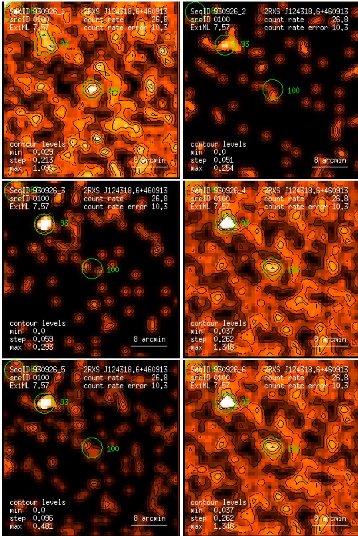
Figure 100: RASS 930926: detection 0100: band rate images, Gaussian filter: (1) PSPC channels 11 – 41, (2) 52 – 90, (3) 91 – 201, (4) 11 – 235, (5) 52 – 201, (6) 11 – 201. Broad band rates in counts/ks. Band rate contour levels in counts/ks/arcmin 2 .
