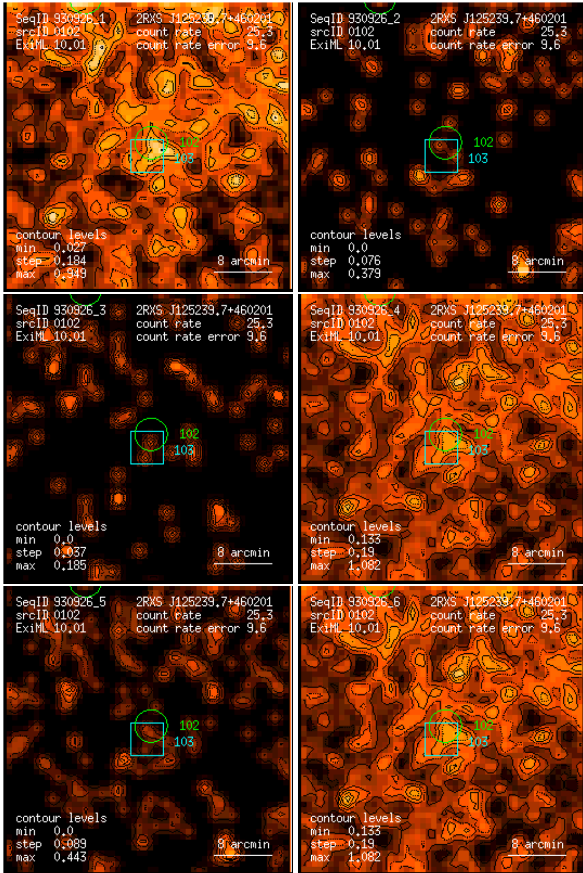
Figure 102: RASS 930926: detection 0102: band rate images, Gaussian filter: (1) PSPC channels 11 – 41, (2) 52 – 90, (3) 91 – 201, (4) 11 – 235, (5) 52 – 201, (6) 11 – 201. Broad band rates in counts/ks. Band rate contour levels in counts/ks/arcmin 2 .
