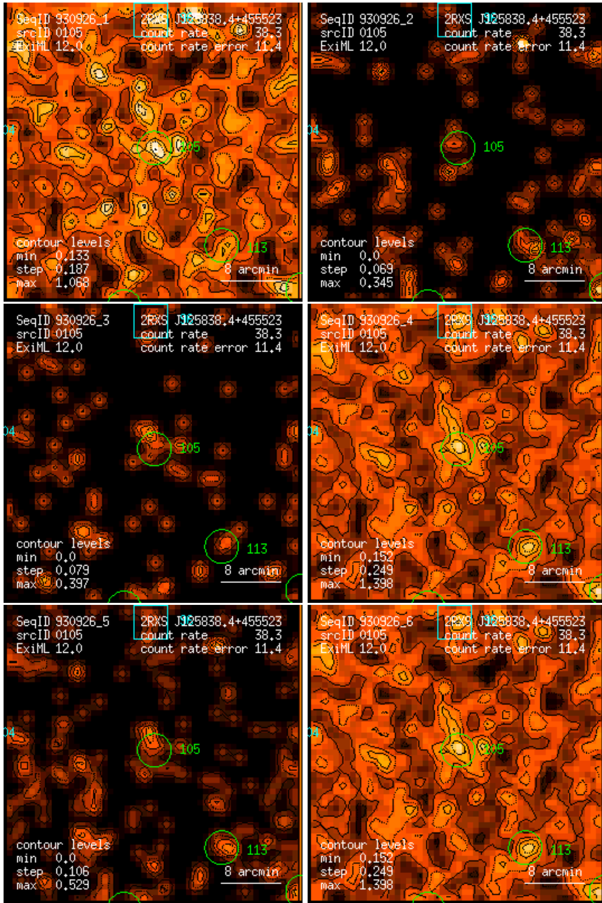
Figure 105: RASS 930926: detection 0105: band rate images, Gaussian filter: (1) PSPC channels 11 – 41, (2) 52 – 90, (3) 91 – 201, (4) 11 – 235, (5) 52 – 201, (6) 11 – 201. Broad band rates in counts/ks. Band rate contour levels in counts/ks/arcmin 2 .
