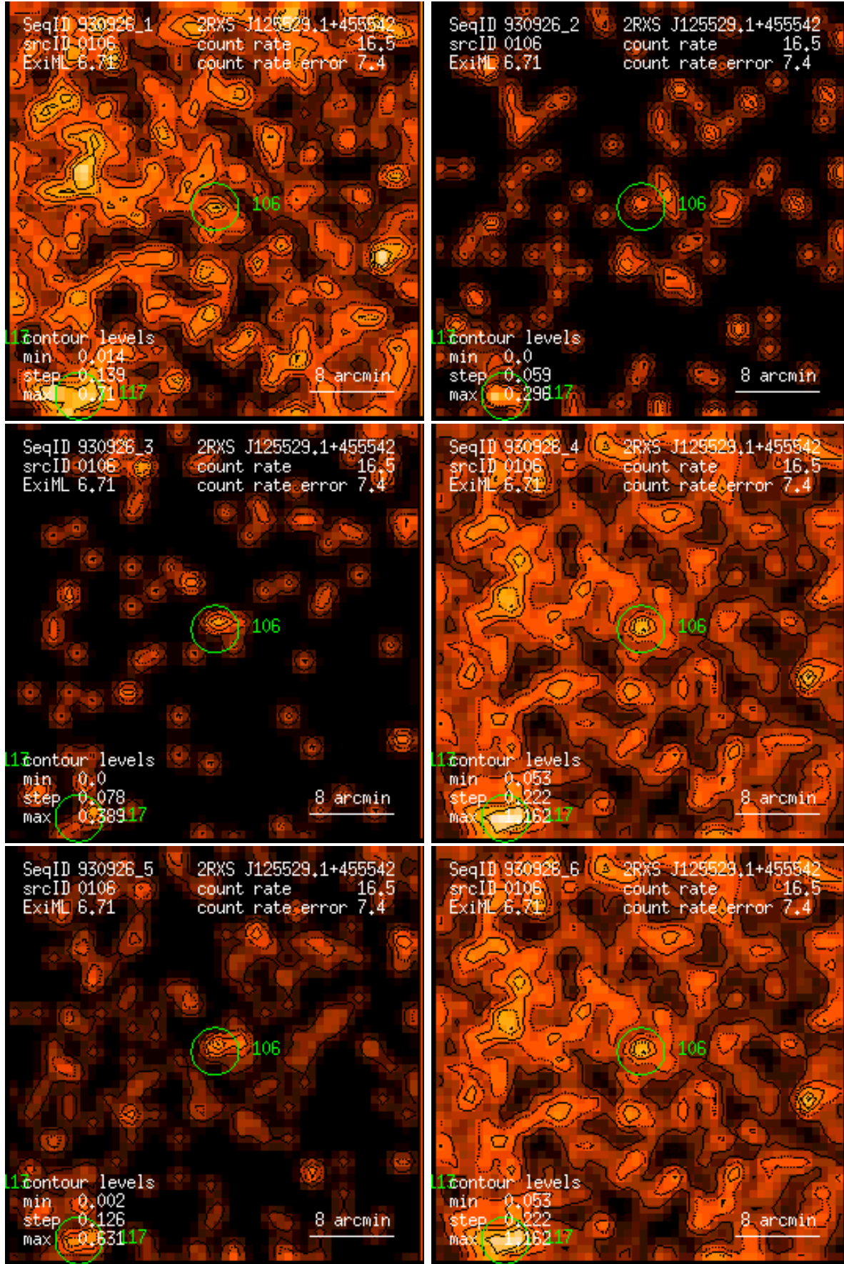
Figure 106: RASS 930926: detection 0106: band rate images, Gaussian filter: (1) PSPC channels 11 – 41, (2) 52 – 90, (3) 91 – 201, (4) 11 – 235, (5) 52 – 201, (6) 11 – 201. Broad band rates in counts/ks. Band rate contour levels in counts/ks/arcmin 2 .
