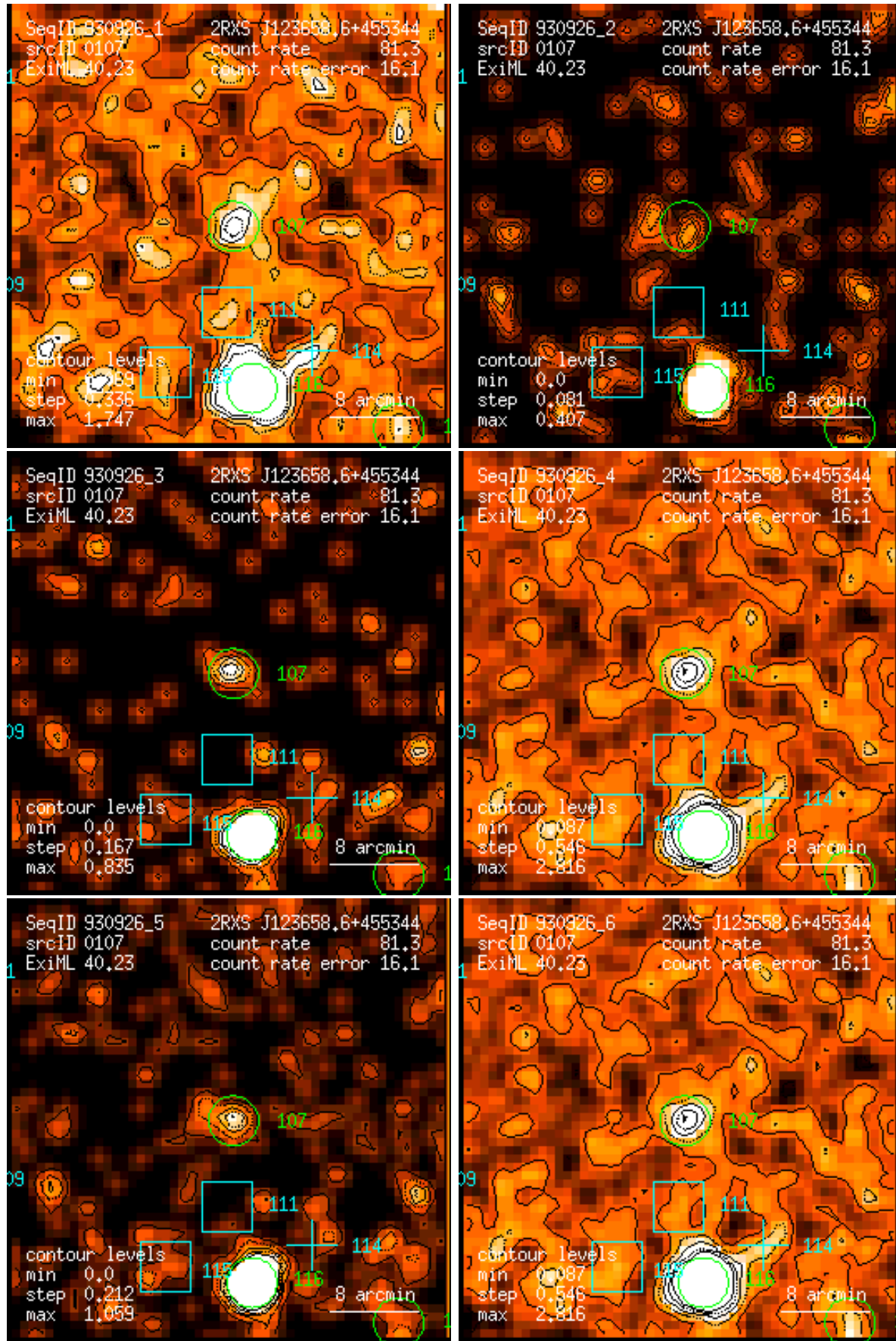
Figure 107: RASS 930926: detection 0107: band rate images, Gaussian filter: (1) PSPC channels 11 – 41, (2) 52 – 90, (3) 91 – 201, (4) 11 – 235, (5) 52 – 201, (6) 11 – 201. Broad band rates in counts/ks. Band rate contour levels in counts/ks/arcmin 2 .
