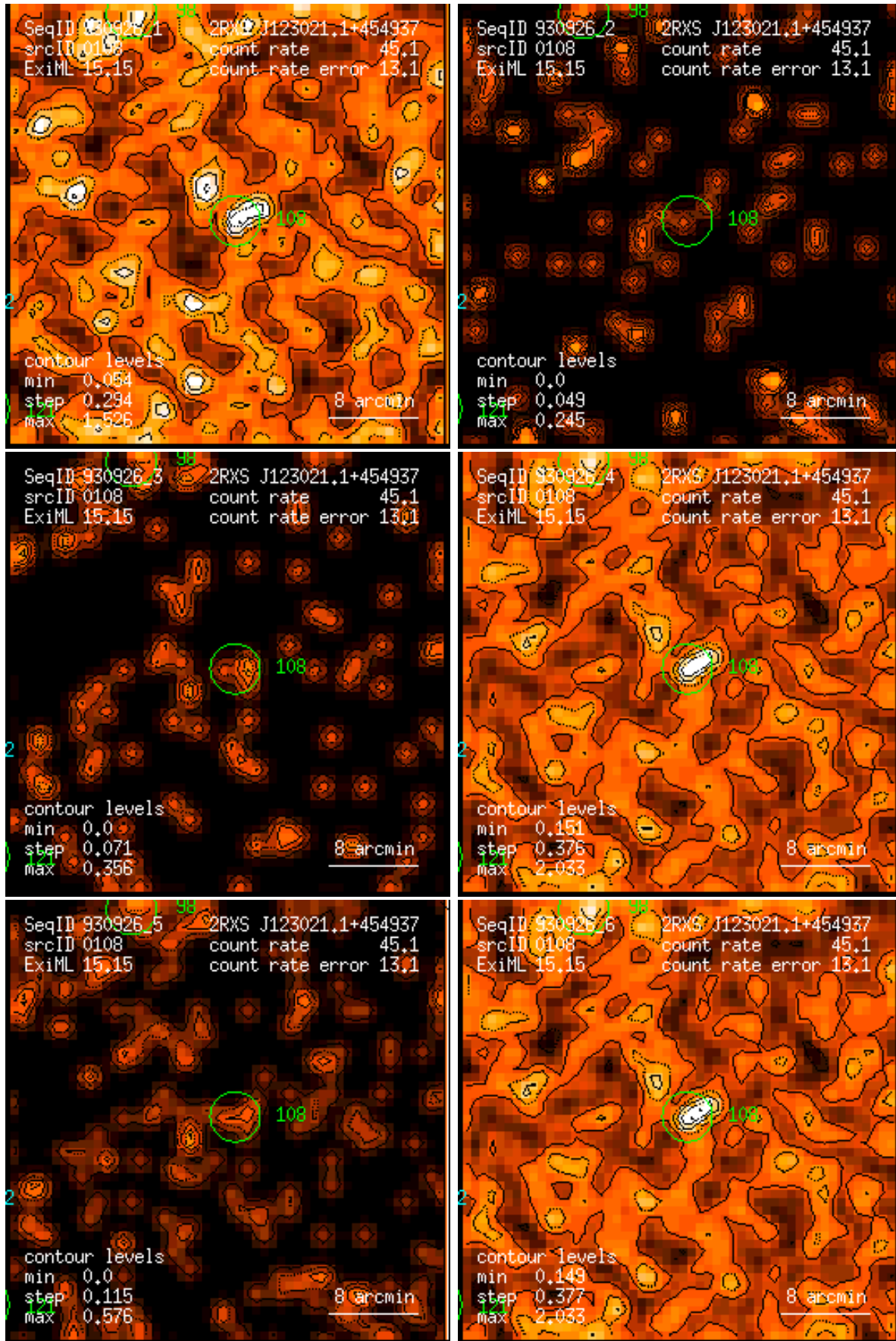
Figure 108: RASS 930926: detection 0108: band rate images, Gaussian filter: (1) PSPC channels 11 – 41, (2) 52 – 90, (3) 91 – 201, (4) 11 – 235, (5) 52 – 201, (6) 11 – 201. Broad band rates in counts/ks. Band rate contour levels in counts/ks/arcmin 2 .
